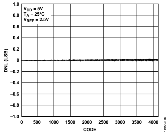
Figure 16. AD5681R DNL
