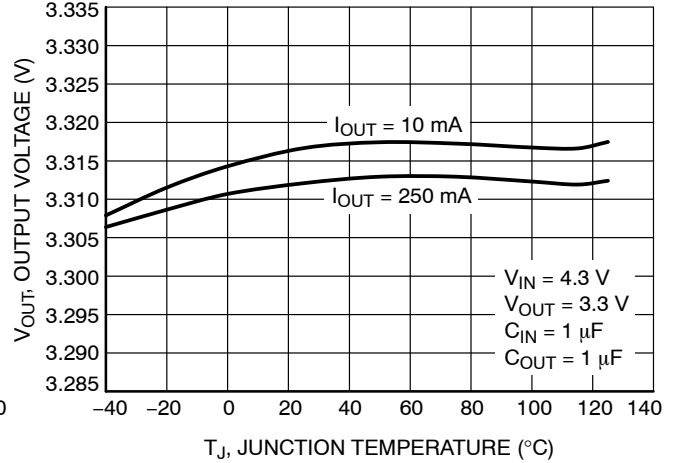
Figure 4. Output Voltage vs. Temperature – V_{OUT} = 3.3\text{ V} – XDFN Package
