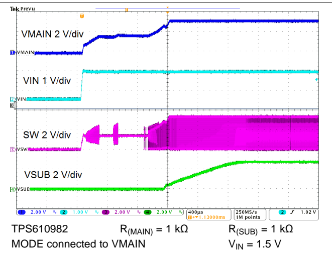
Figure 95. Startup
