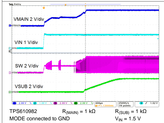
Figure 94. Startup
