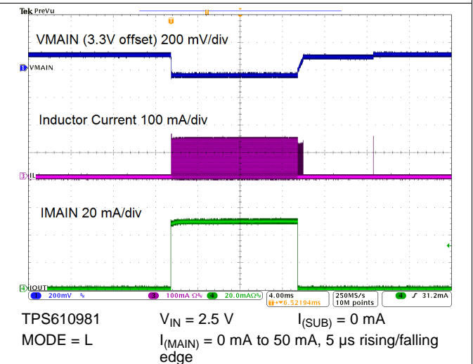
Figure 68. Load Transient Response
