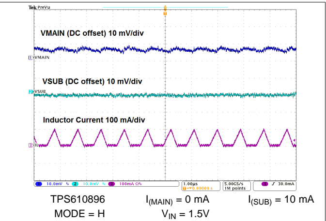
Figure 66. Switching Waveforms
