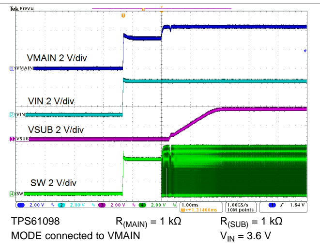
Figure 93. Startup
