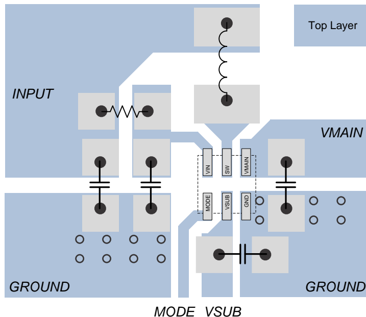
Figure 96. Layout
