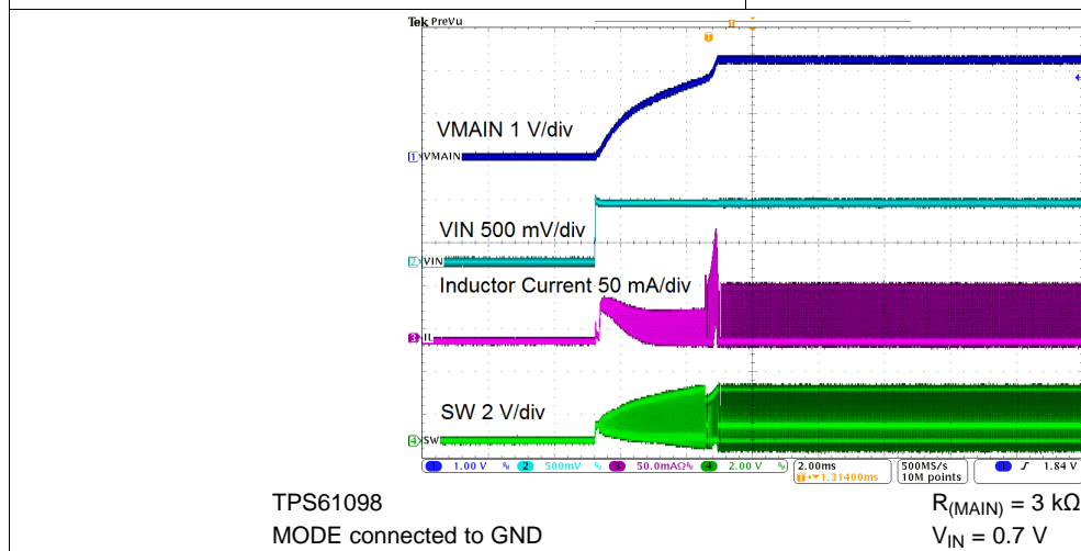
Figure 84. Startup
