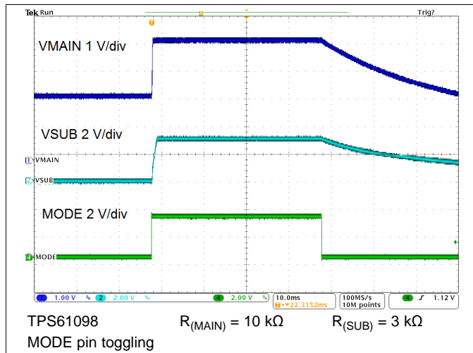
Figure 92. MODE Toggling
