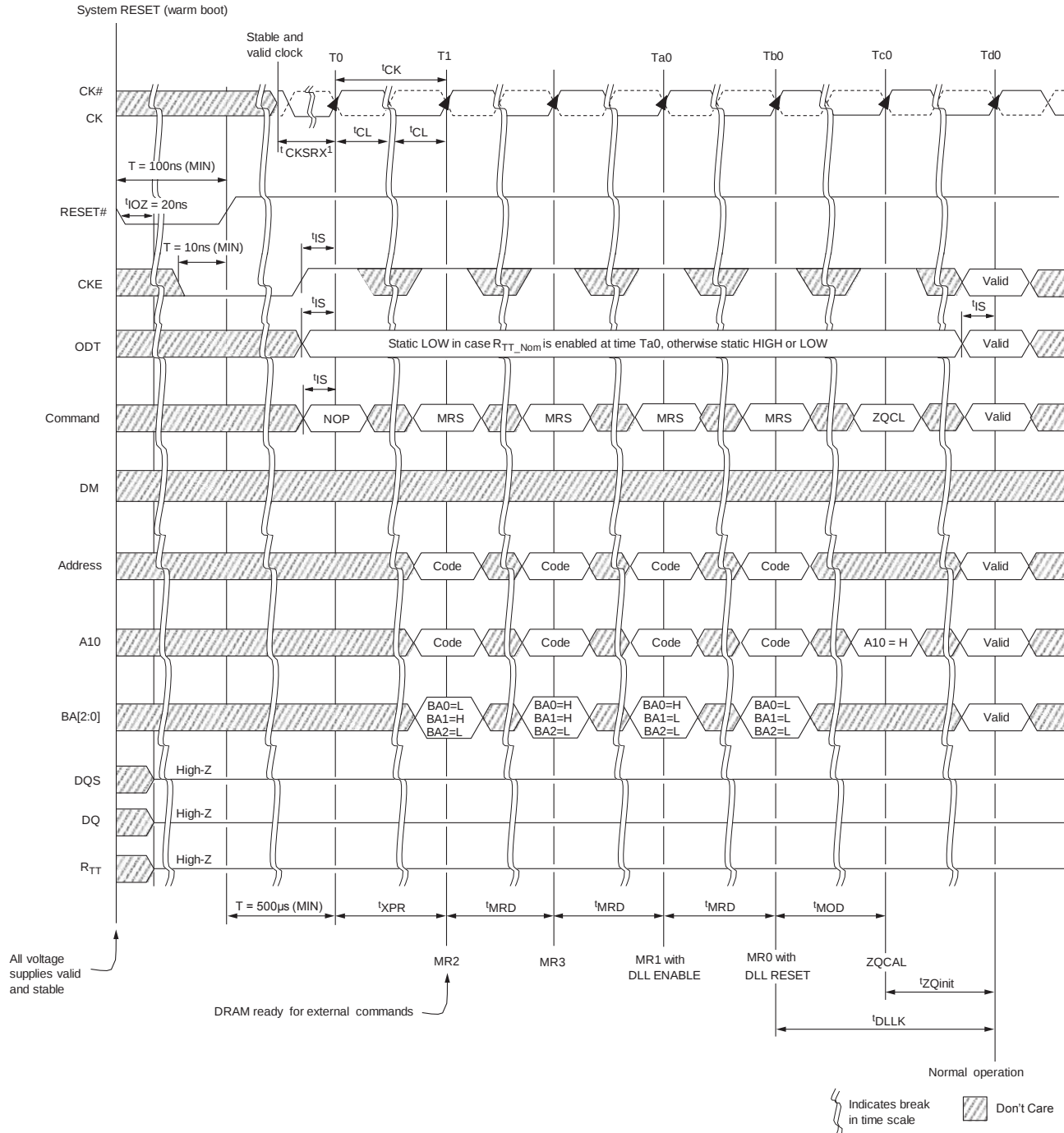
Figure 96 : RESET Sequence
