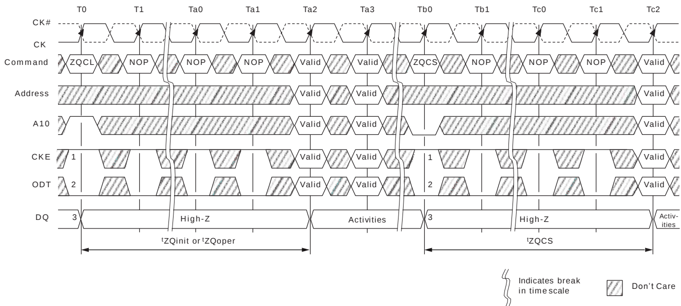
Figure 53 : ZQ CALIBRATION Timing (ZQCL and ZQCS)
