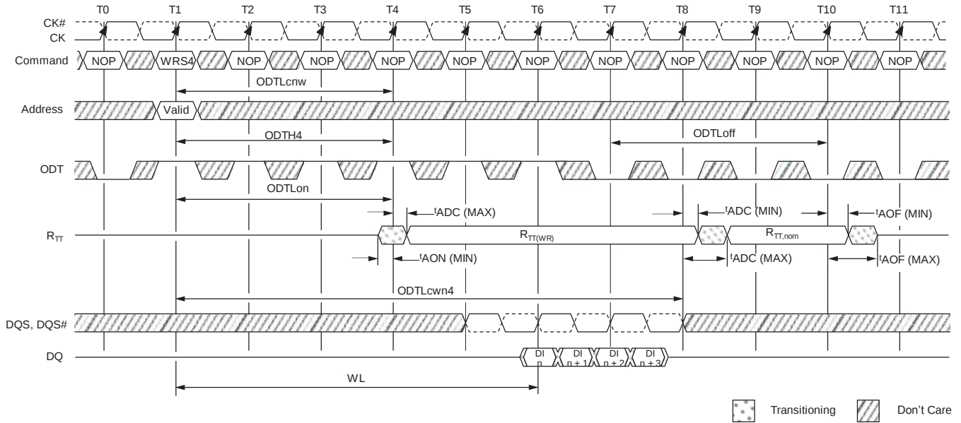
Figure 101 : Dynamic ODT: ODT Pin Asserted with WRITE Command for 6 Clock Cycles, BC4
