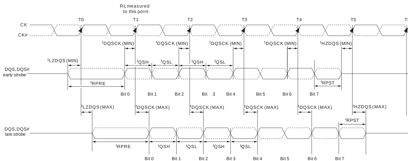
Figure 67 : Data Strobe Timing – READs
