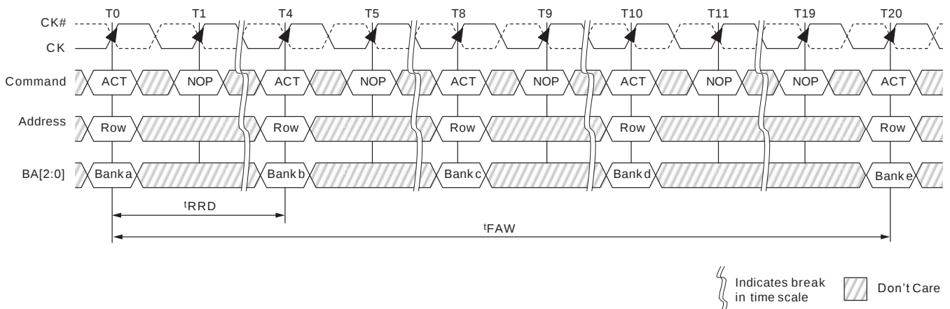
Figure 55 : Example: t_{FAW}
