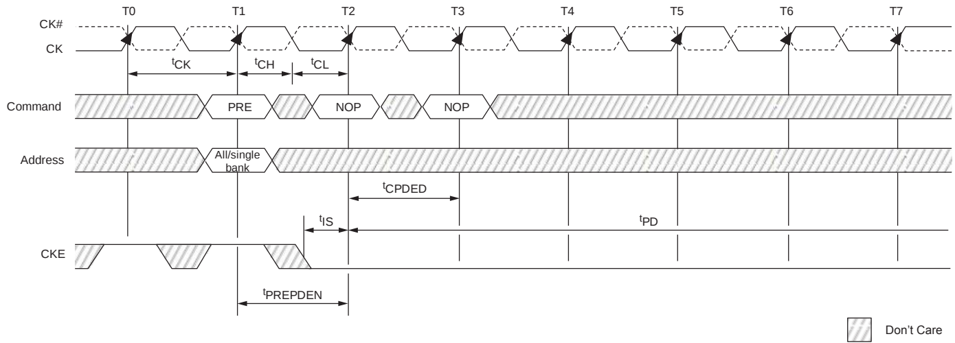
Figure 93 : PRECHARGE to Power-Down Entry
