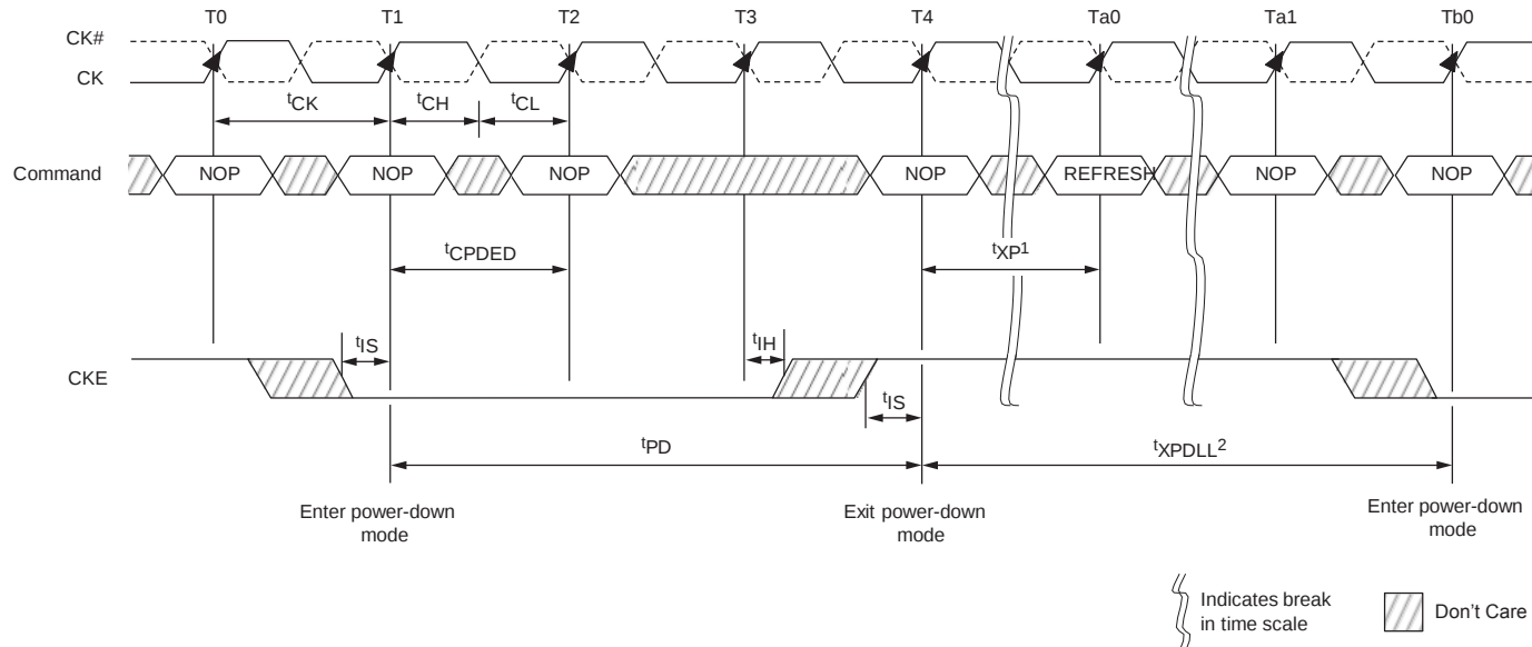
Figure 95 : Power-Down Exit to Refresh to Power-Down Entry
