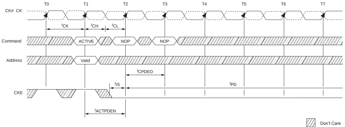
Figure 92 : ACTIVATE to Power-Down Entry
