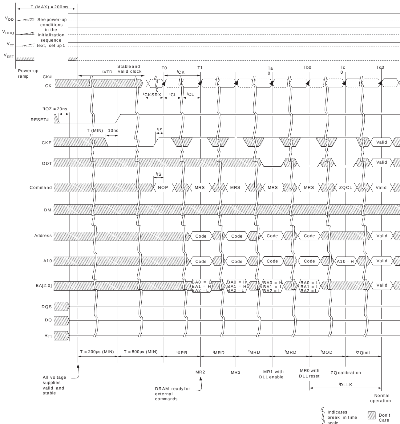
Figure 37 : Initialization Sequence
