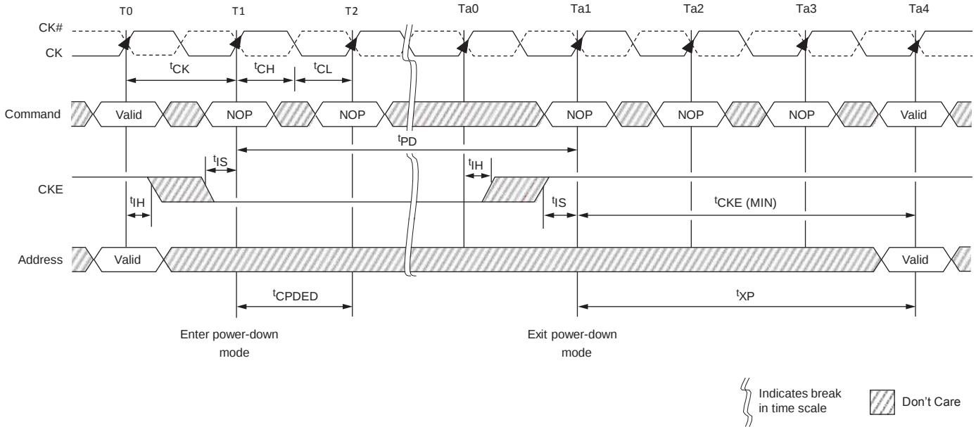
Figure 85 : Active Power-Down Entry and Exit
