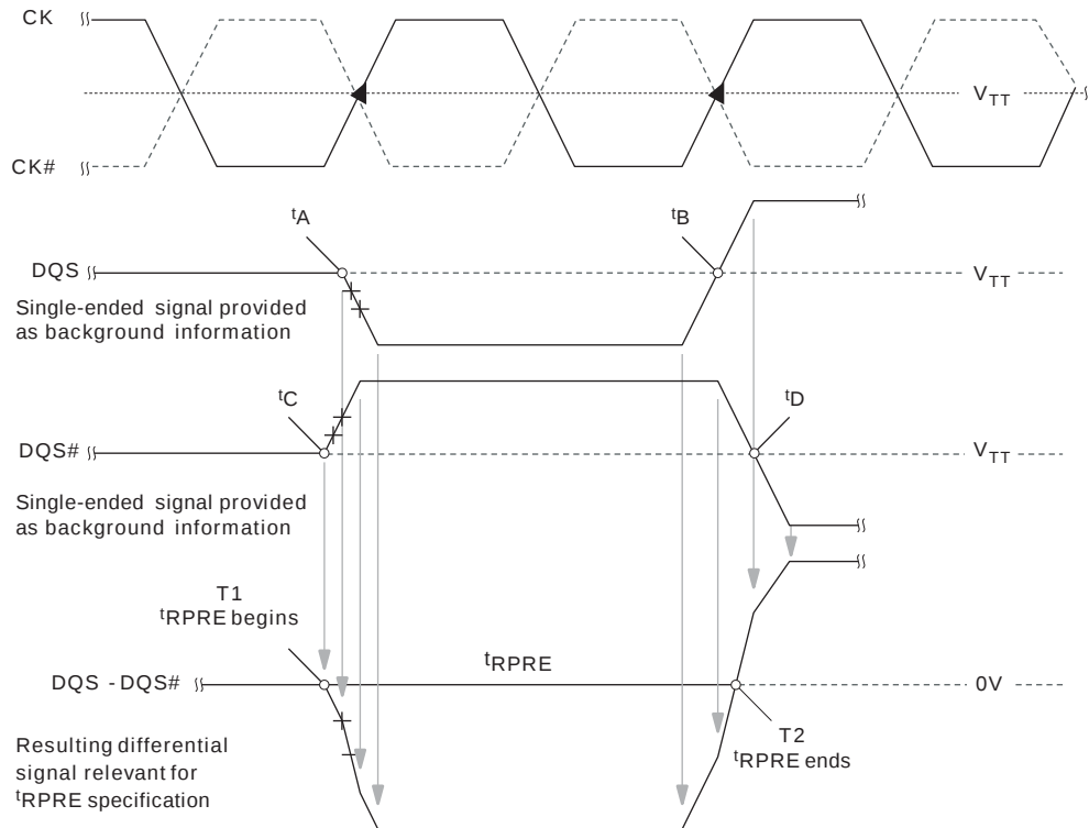
Figure 69 : tRPRE Timing
