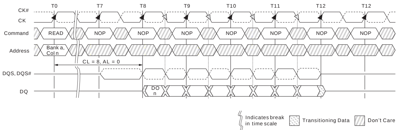
Figure 56 : READ Latency
