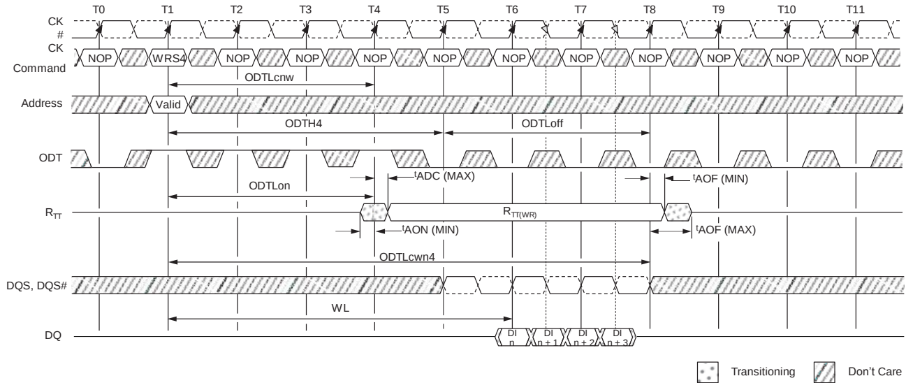
Figure 102 : Dynamic ODT: ODT Pin Asserted with WRITE Command for 4 Clock Cycles, BC4
