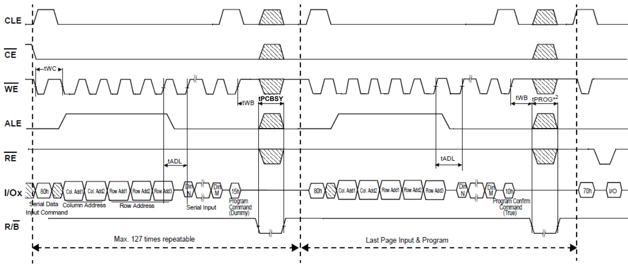
Figure 20 : cache program
