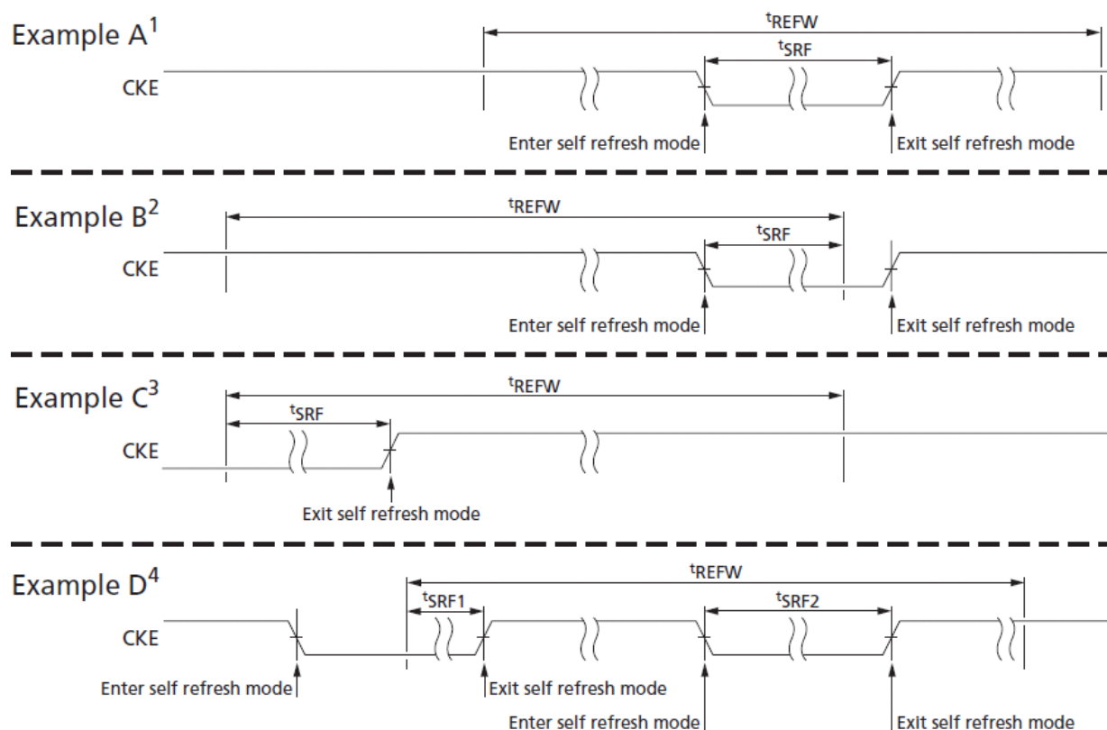
Figure 32: tSRF Definition
