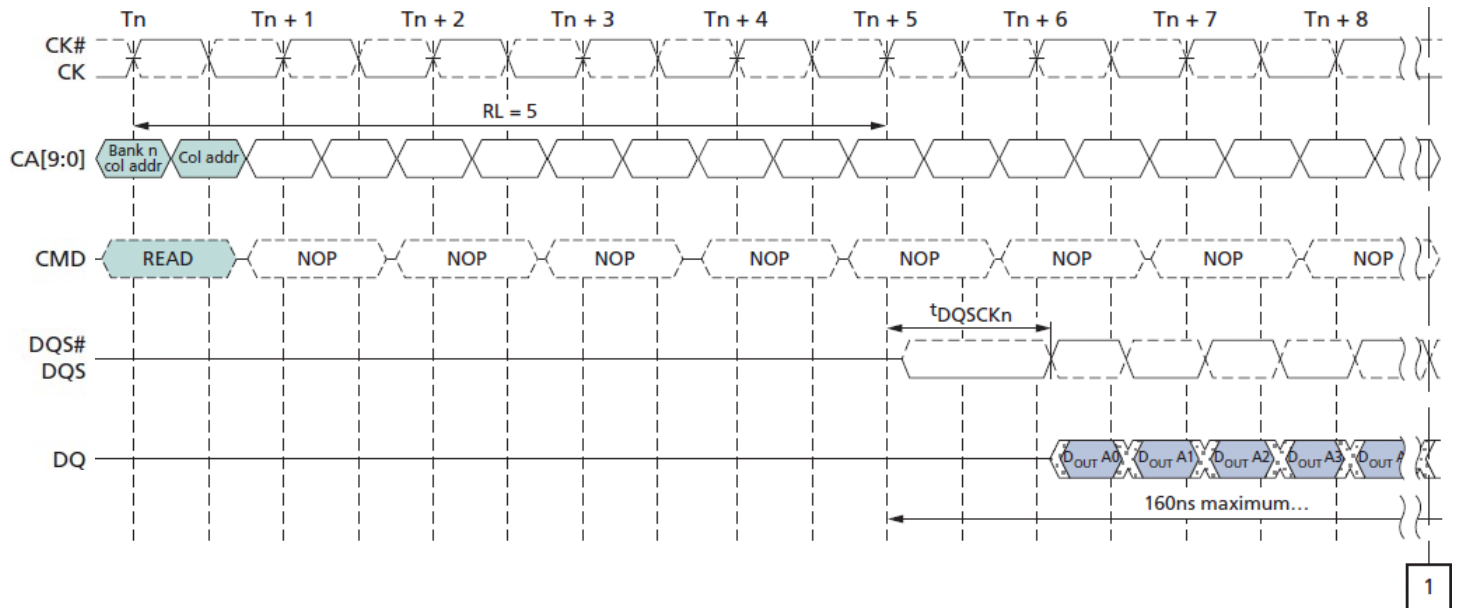
Figure 10 : tDQCKDS Timing
