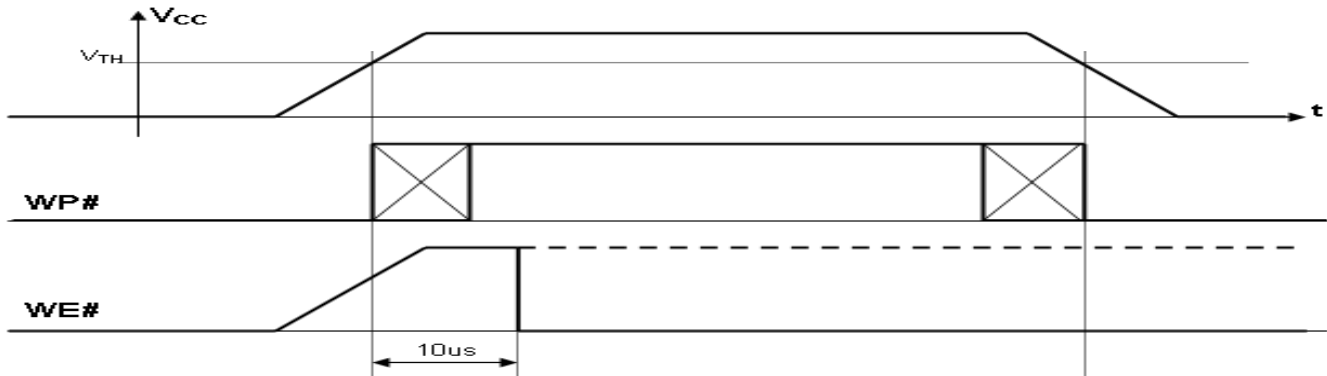
Figure 31 : Power on and Data Protection timings
