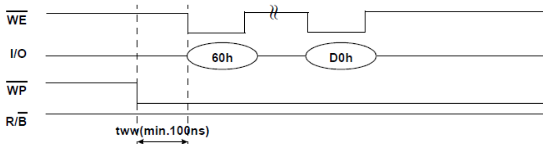
Figure 30 : t_{WW} in Erase Operation
