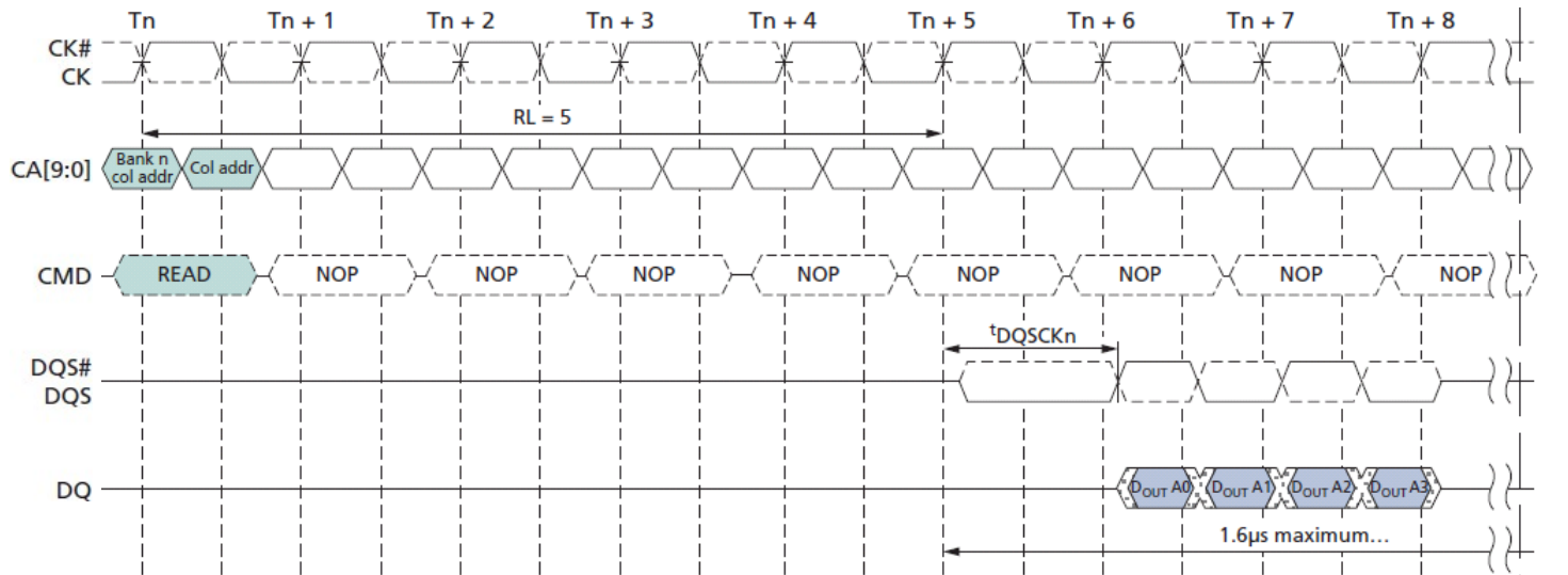
Figure 9 : tDQCKDM Timing
