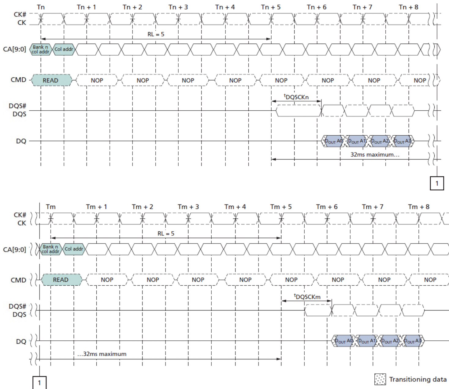
Figure 8 : tDQSCKDL Timing
