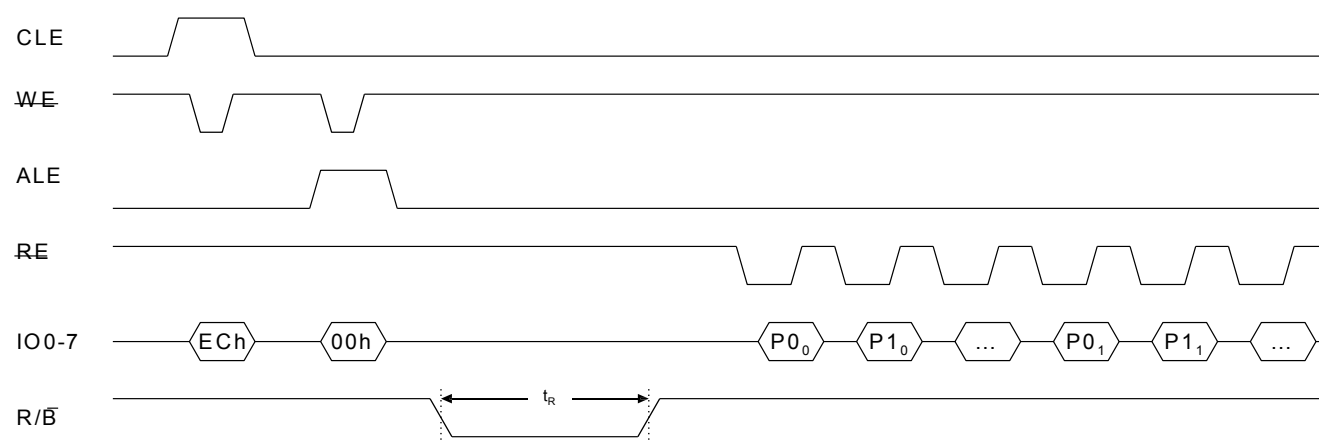
Figure 28 : Read Parameter Page timings
