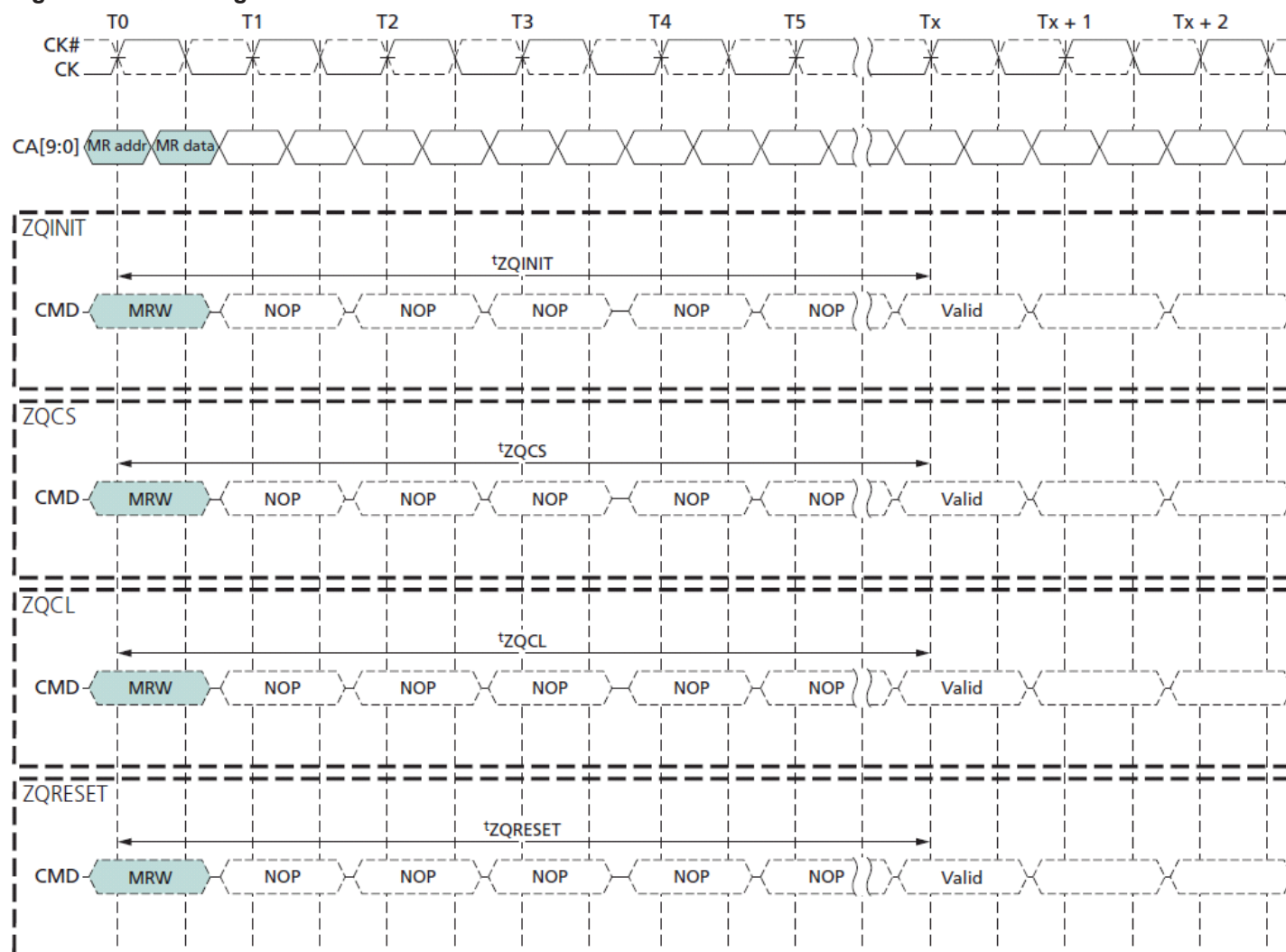
Figure 42: ZQ Timings
