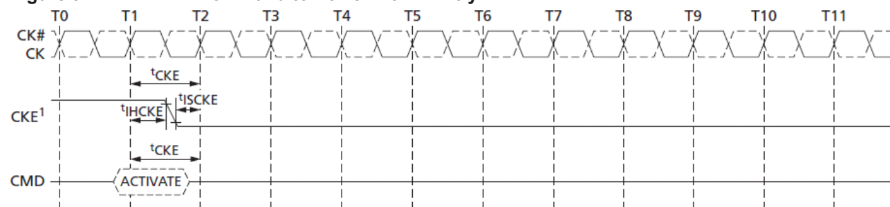
Figure 51: ACTIVATE Command to Power-Down Entry
