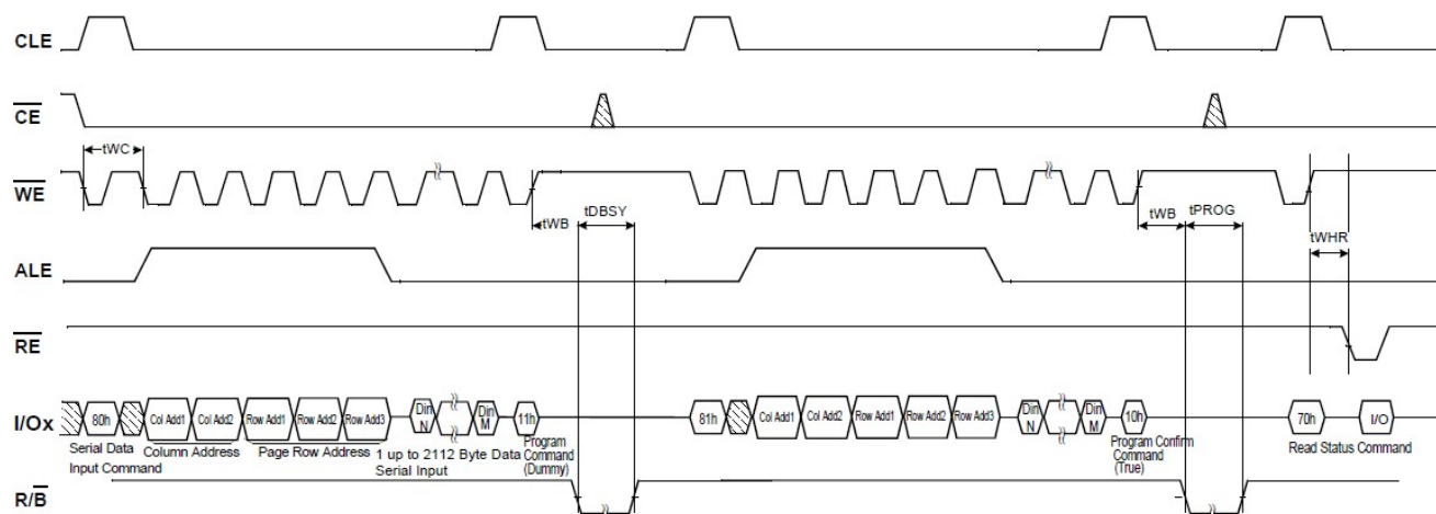
Figure 17 : multi-plane program
