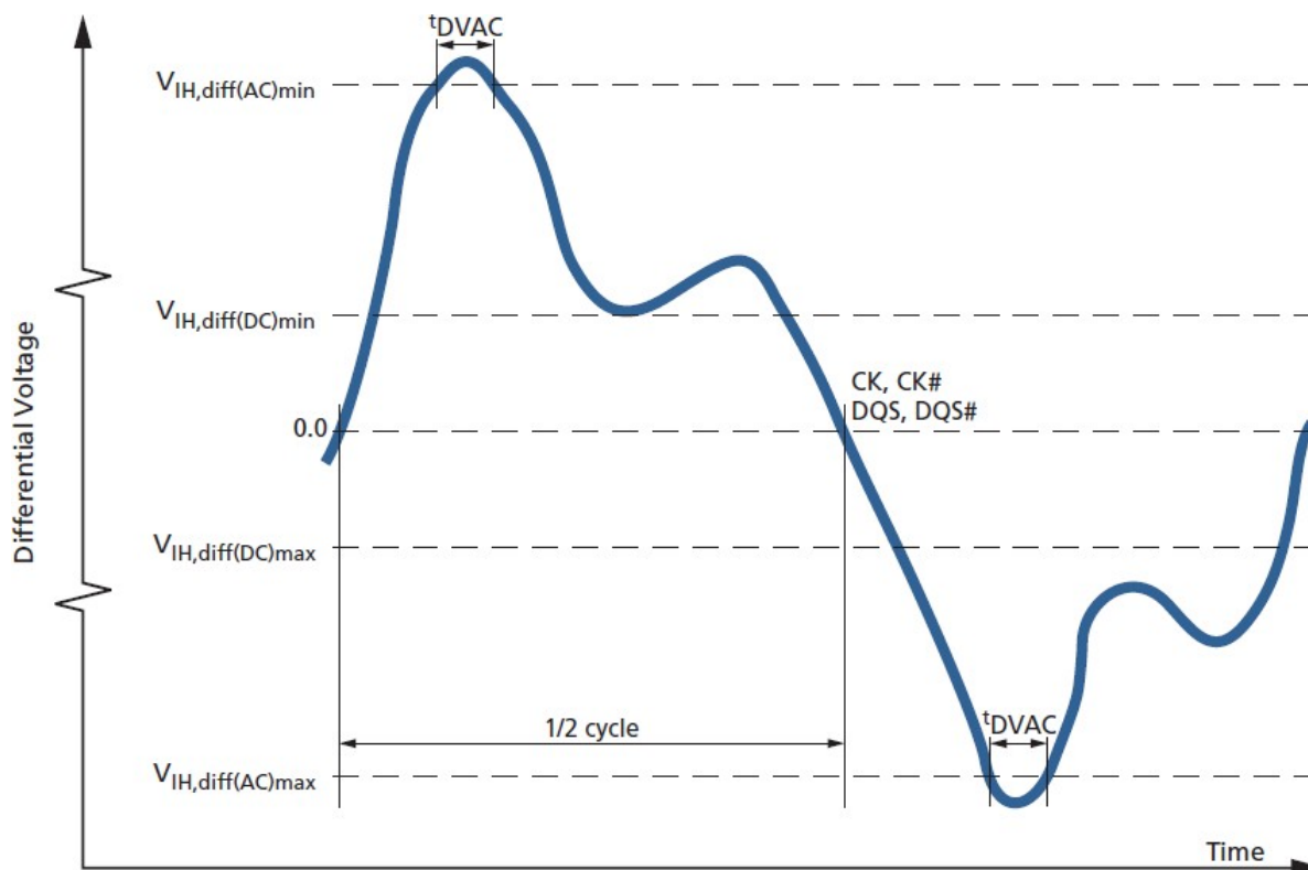
Figure 59: Differential AC Swing Time and t_{DVAC}
