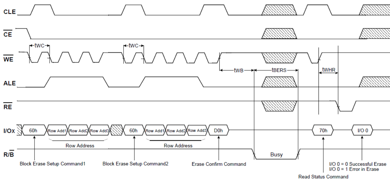
Figure 23 : multi-plane block erase
