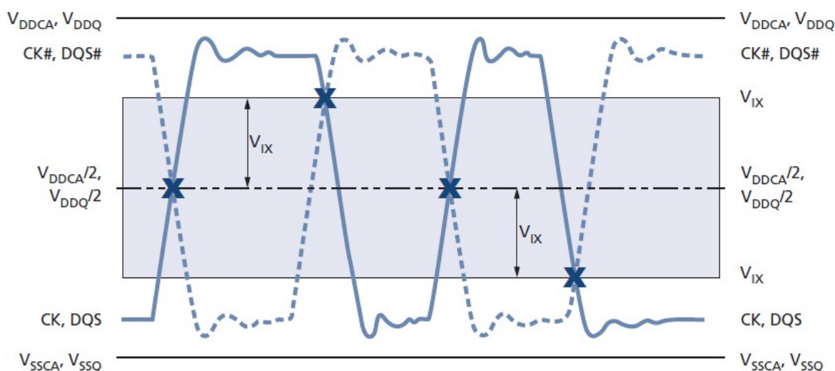
Figure 61: V_{IX} Definition
