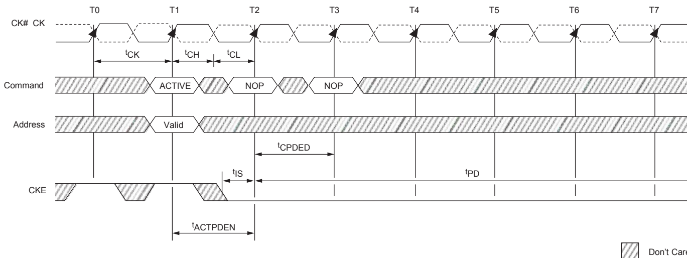
Figure 92 : ACTIVATE to Power-Down Entry
