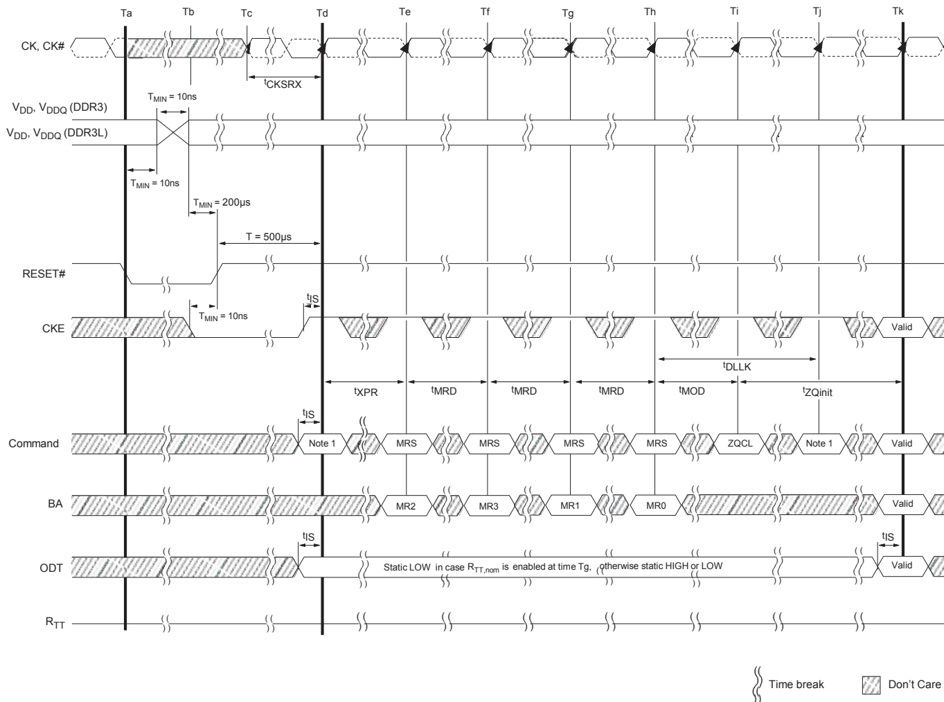
Figure 38 : V DD Voltage Switching
