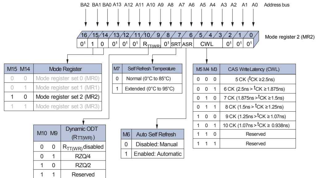
Figure 45 : Mode Register 2 (MR2) Definition
