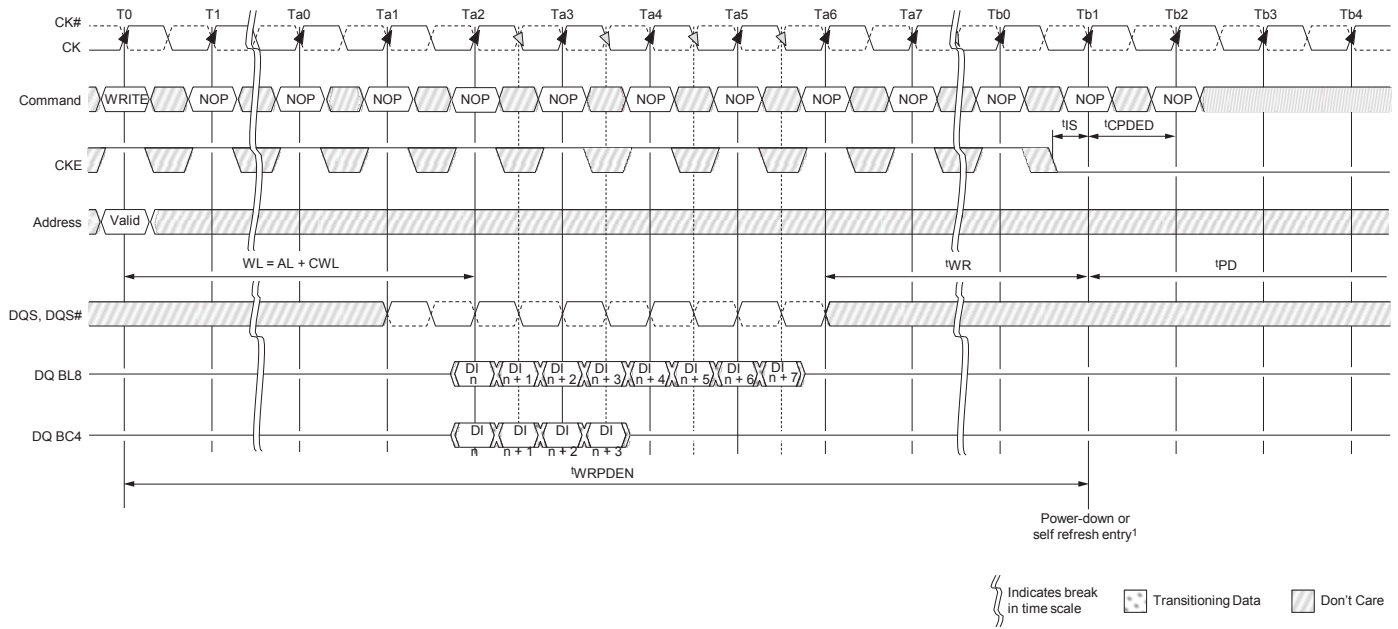
Figure 89 : Power-Down Entry After WRITE
