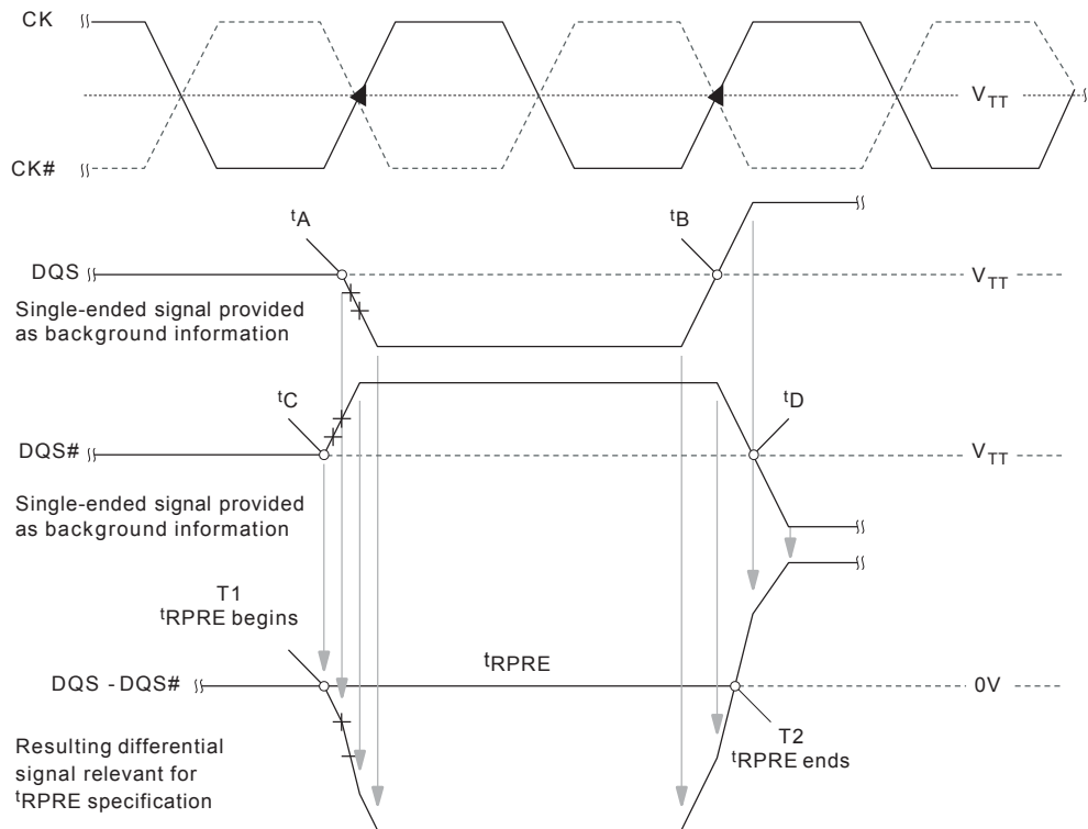
Figure 69 : tRPRE Timing
