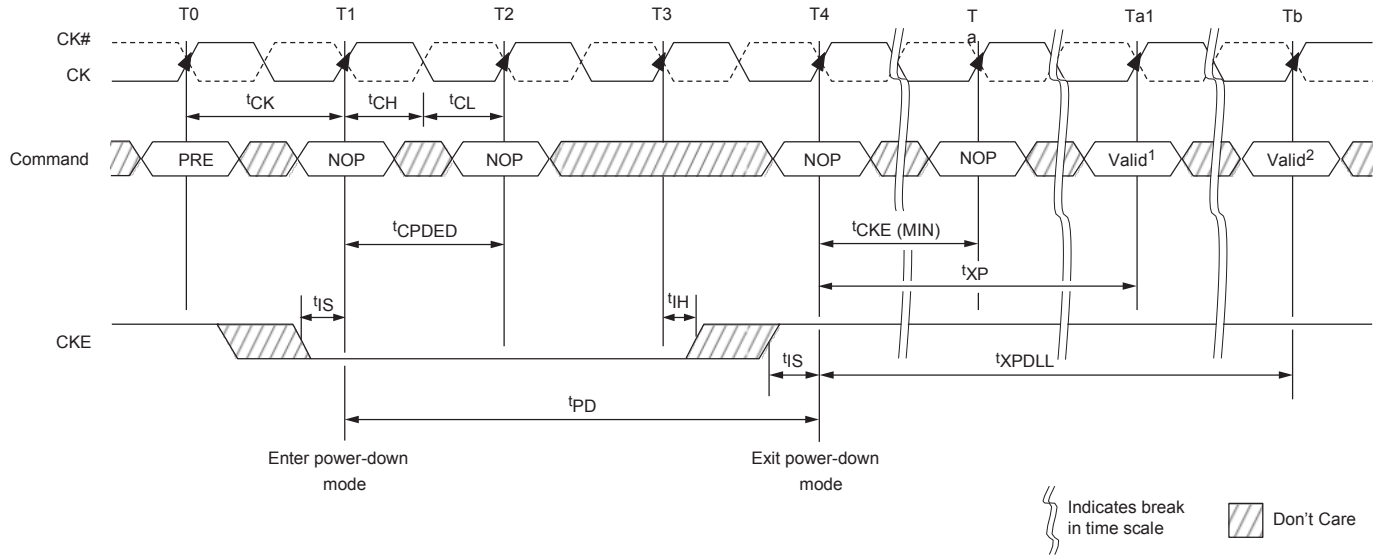
Figure 87 : Precharge Power-Down (Slow-Exit Mode) Entry and Exit
