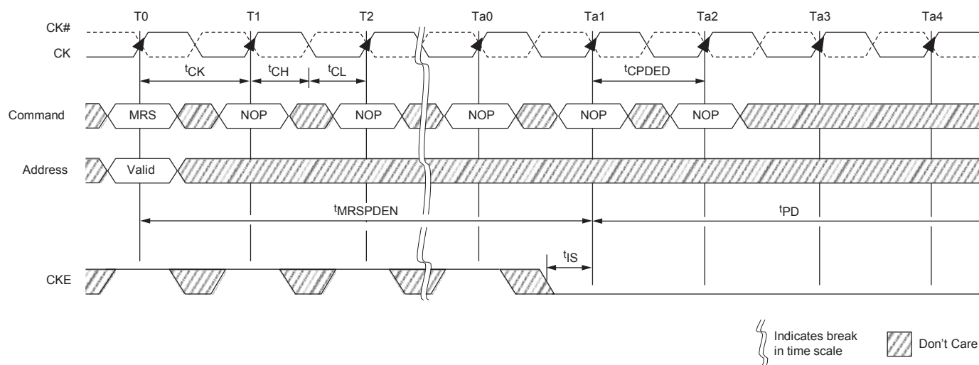
Figure 94 : MRS Command to Power-Down Entry
