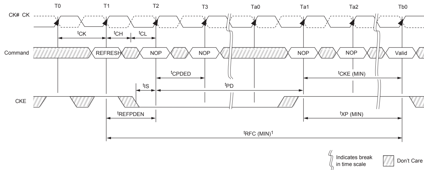
Figure 91 : REFRESH to Power-Down Entry
