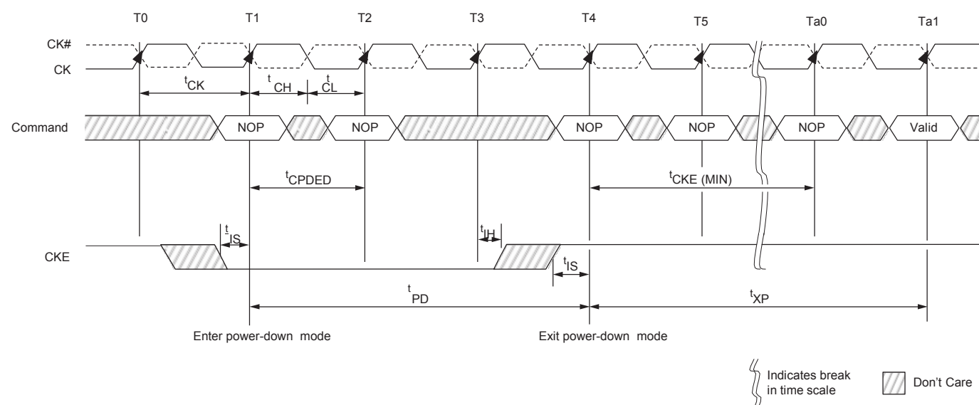
Figure 86 : Precharge Power-Down (Fast-Exit Mode) Entry and Exit
