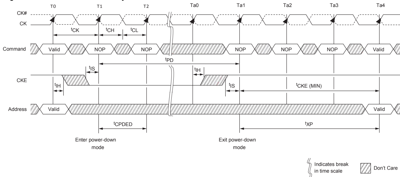
Figure 85 : Active Power-Down Entry and Exit
