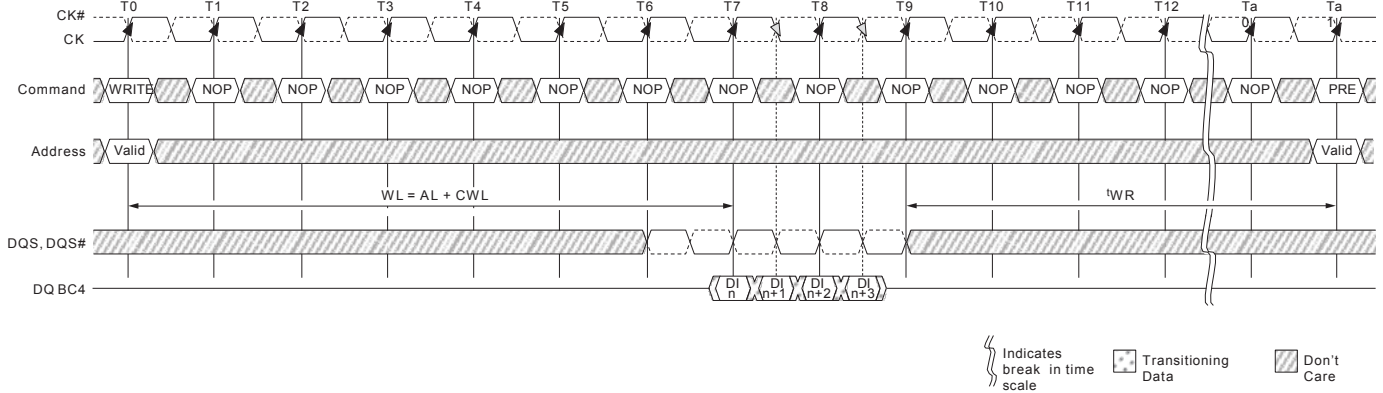
Figure 81 : WRITE (BC4 Mode Register Setting) to PRECHARGE
