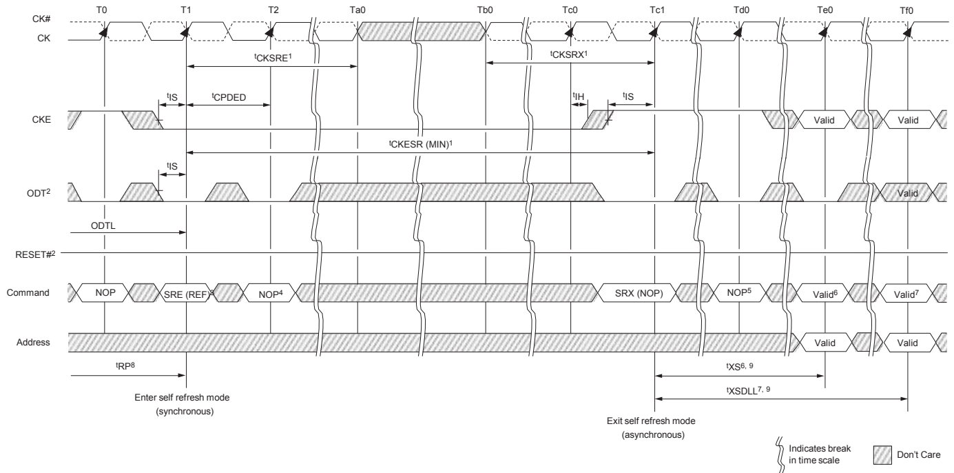
Figure 84 : Self Refresh Entry/Exit Timing
