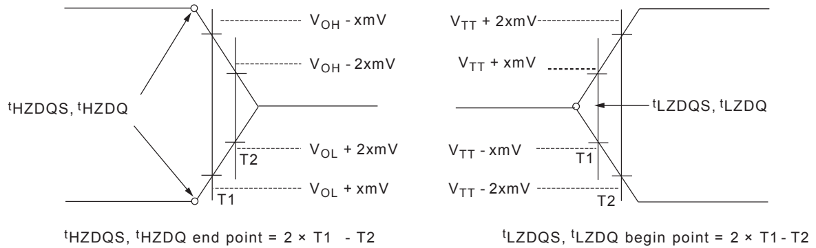
Figure 68 : Method for Calculating tLZ and tHZ
