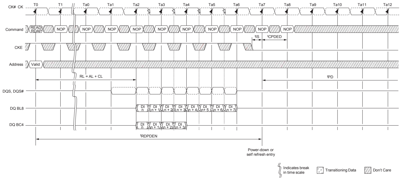
Figure 88 : Power-Down Entry After READ or READ with Auto Precharge (RDAP)
