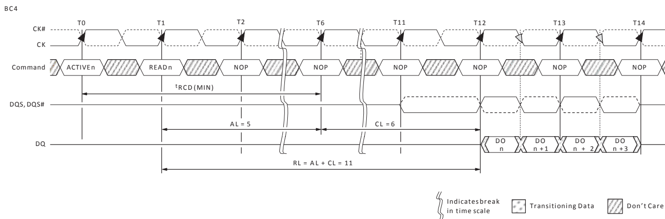
Figure 44 : READ Latency (AL = 5, CL = 6)
