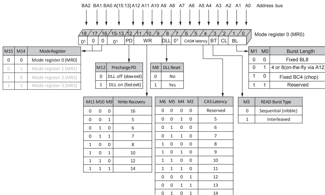
Figure 41 : Mode Register 0 (MR0) Definitions
