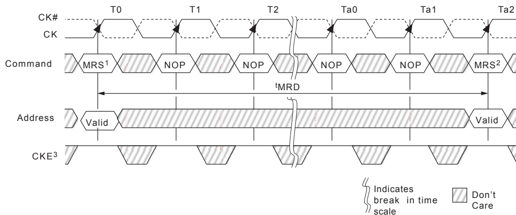
Figure 39 : MRS to MRS Command Timing ( t_{MRD} )
