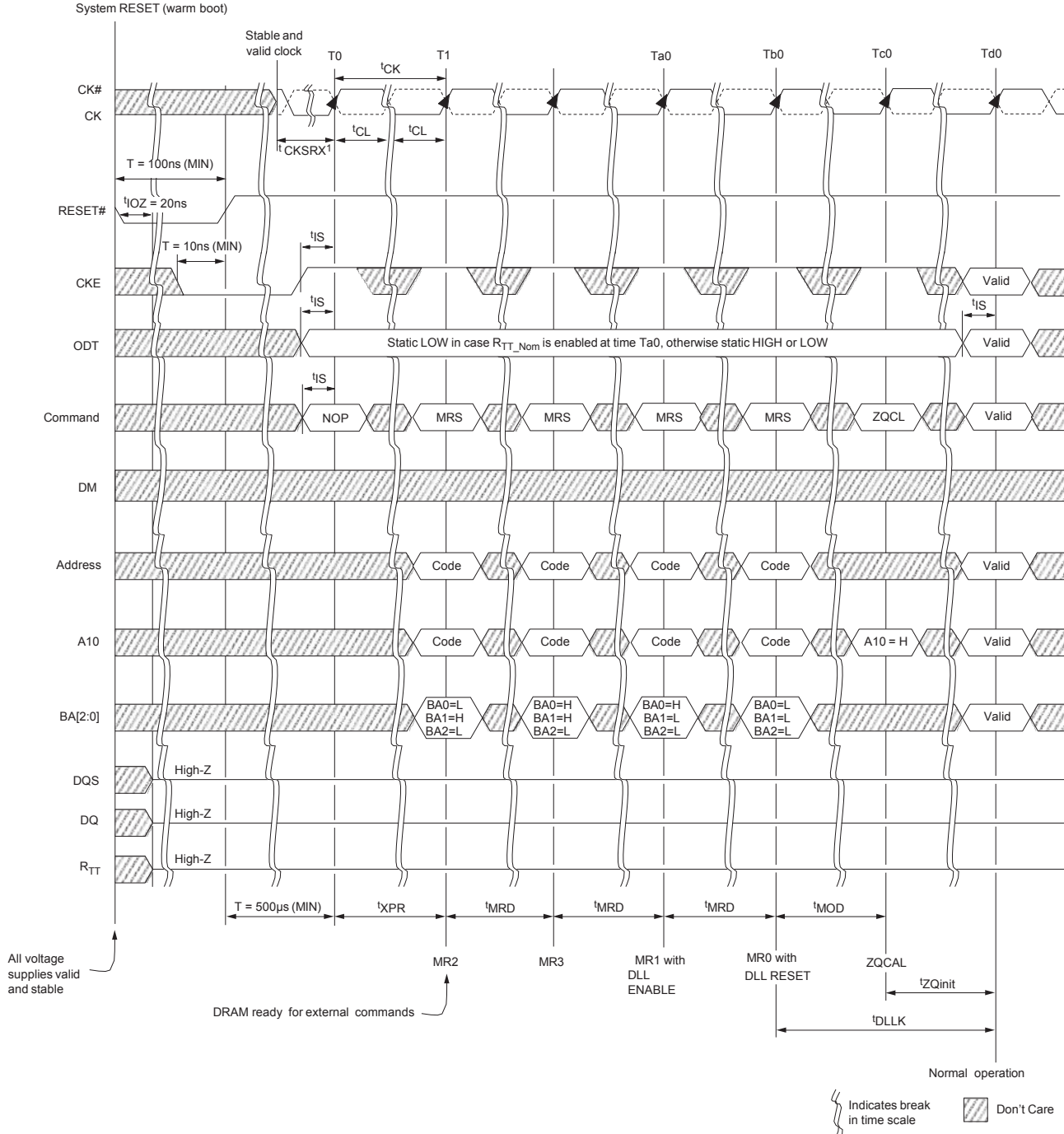
Figure 96 : RESET Sequence
