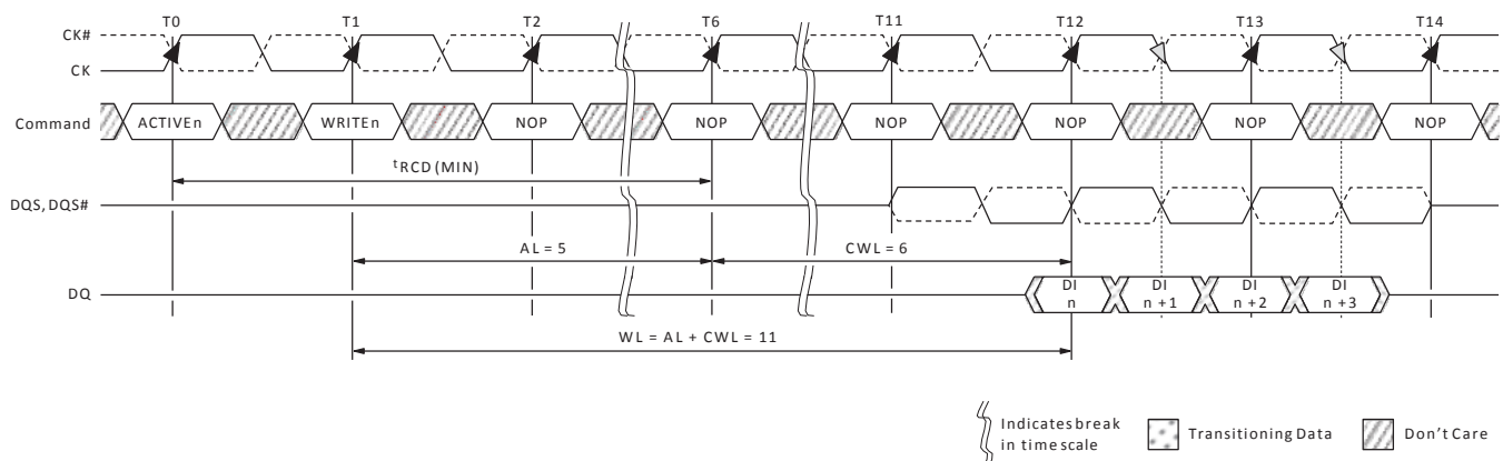
Figure 46 : CAS Write Latency
