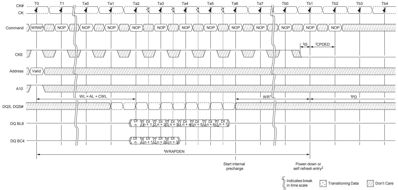
Figure 90 : Power-Down Entry After WRITE with Auto Precharge (WRAP)
