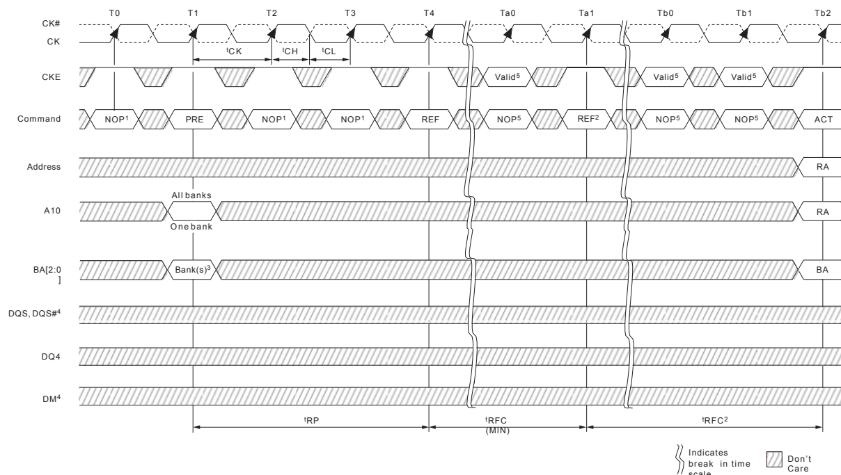
Figure 29 : Refresh Mode
