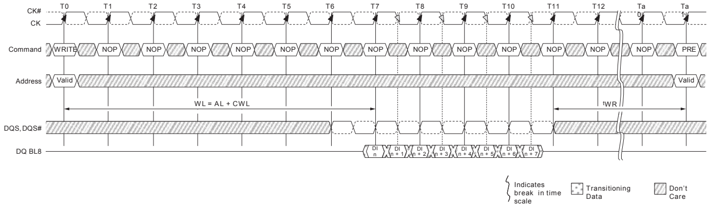
Figure 80 : WRITE (BL8) to PRECHARGE
