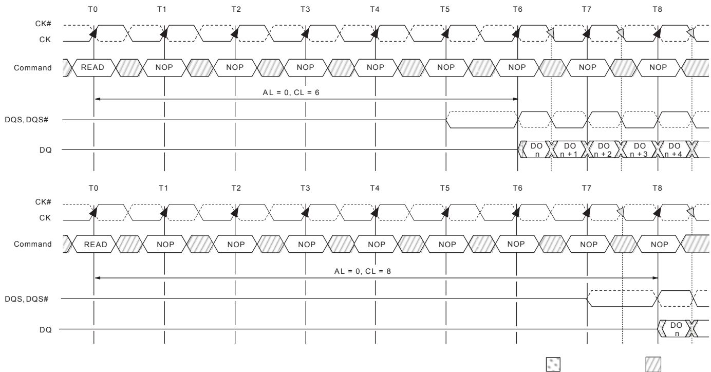
Figure 42 : READ Latency
