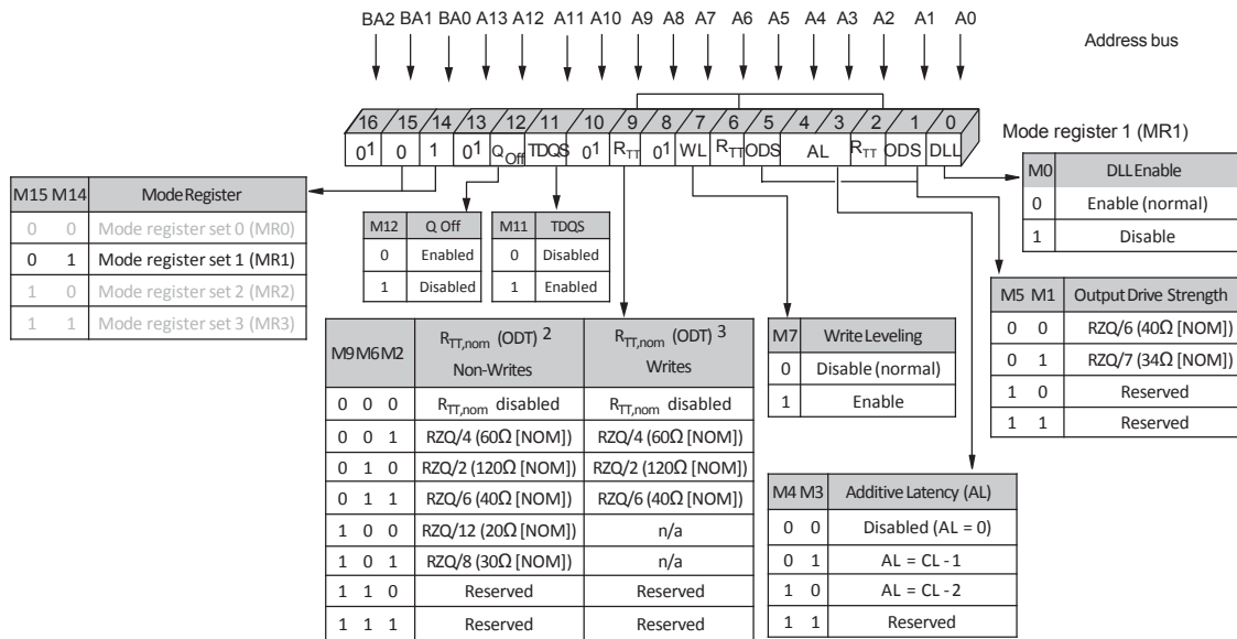
Figure 43 : Mode Register 1 (MR1) Definition
