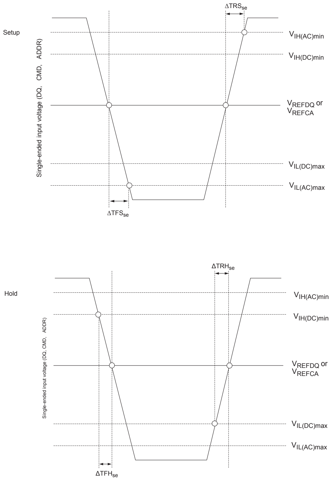
Figure 8 : Nominal Slew Rate Definition for Single-Ended Input Signals
