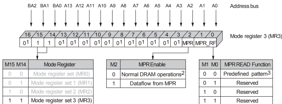
Figure 47 : Mode Register 3 (MR3) Definition
