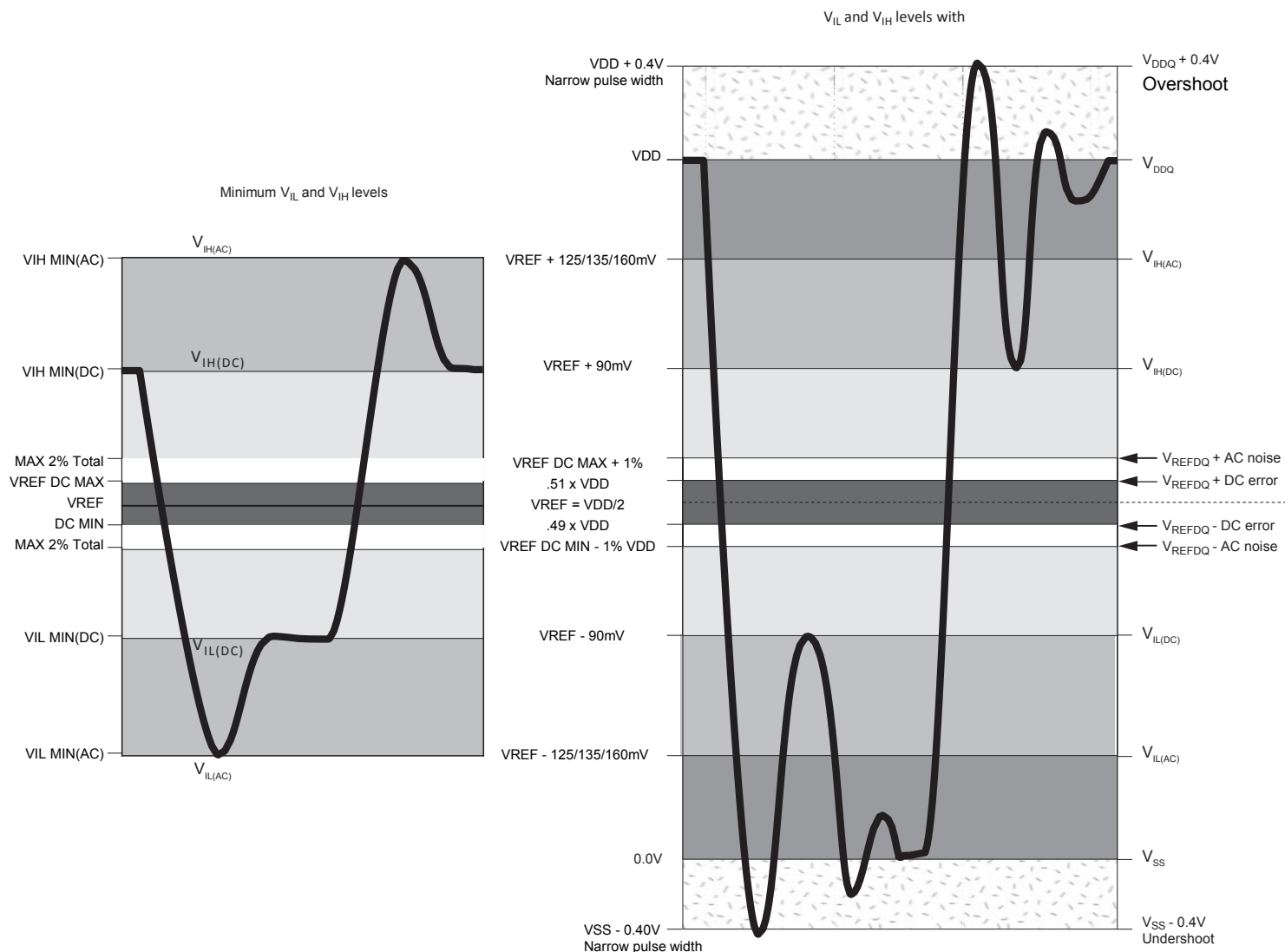
Figure 2 : DDR3L 1.35V Input Signal
