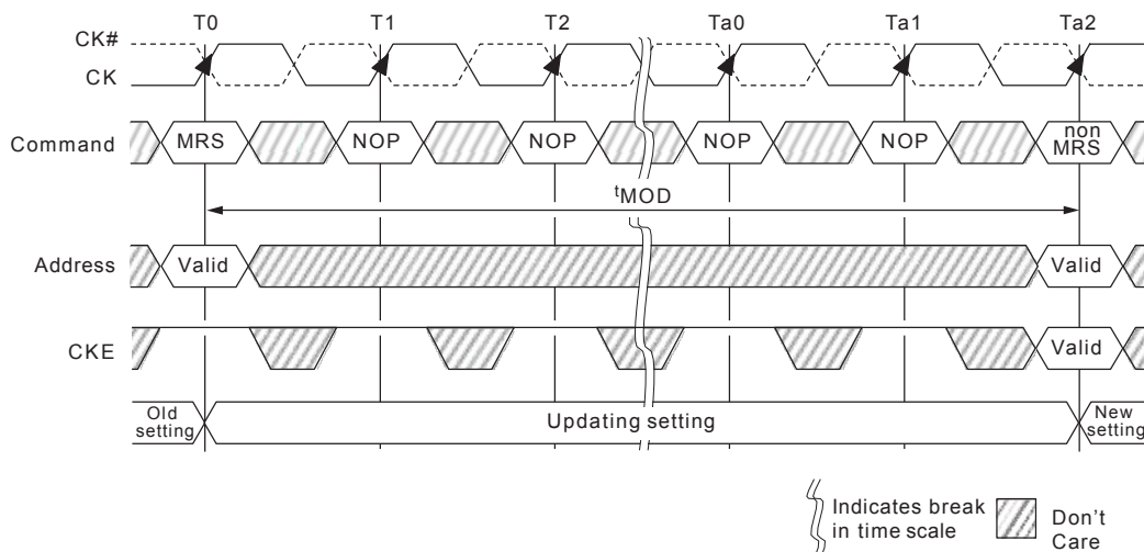
Figure 40 : MRS to nonMRS Command Timing (tMOD)
