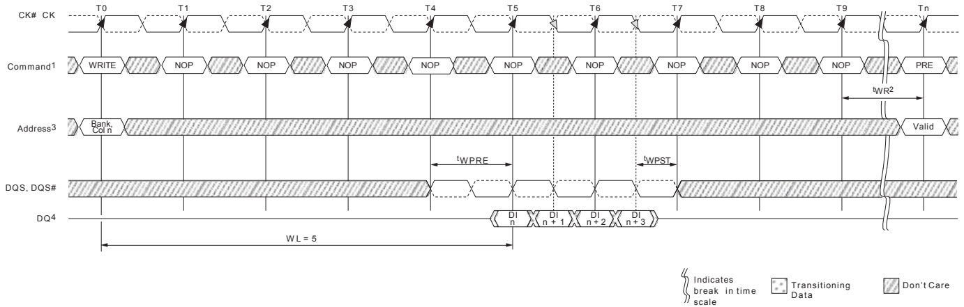
Figure 82 : WRITE (BC4 OTF) to PRECHARGE
