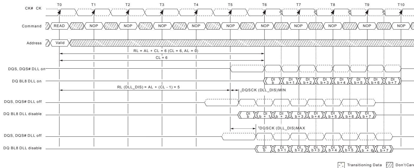
Figure 32 : DLL Disable tDQSK
