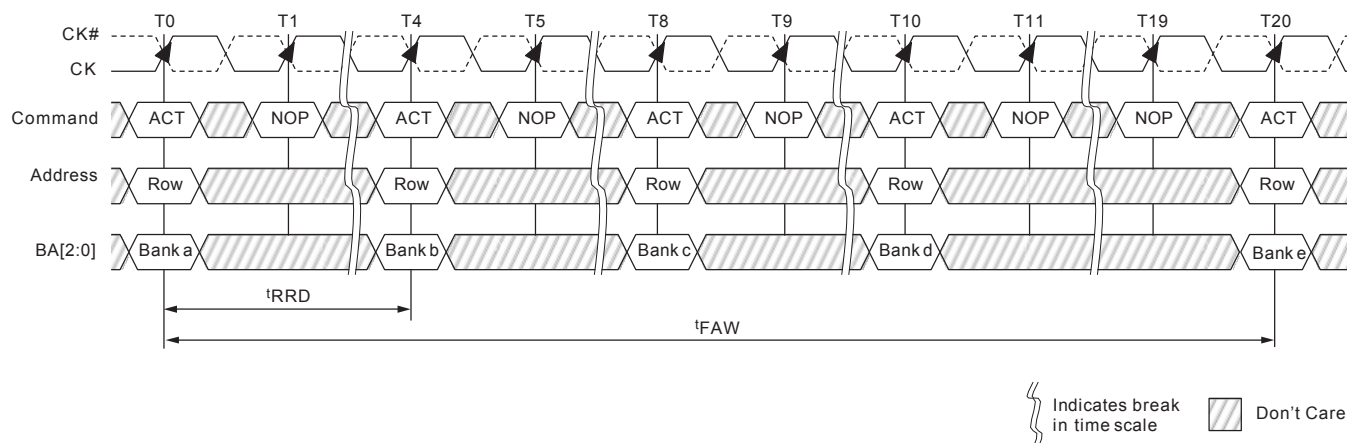
Figure 55 : Example: t_{FAW}
