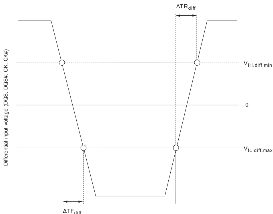
Figure 9 : DDR3L 1.35V Nominal Differential Input Slew Rate Definition for DQS, DQS# and CK, CK#
