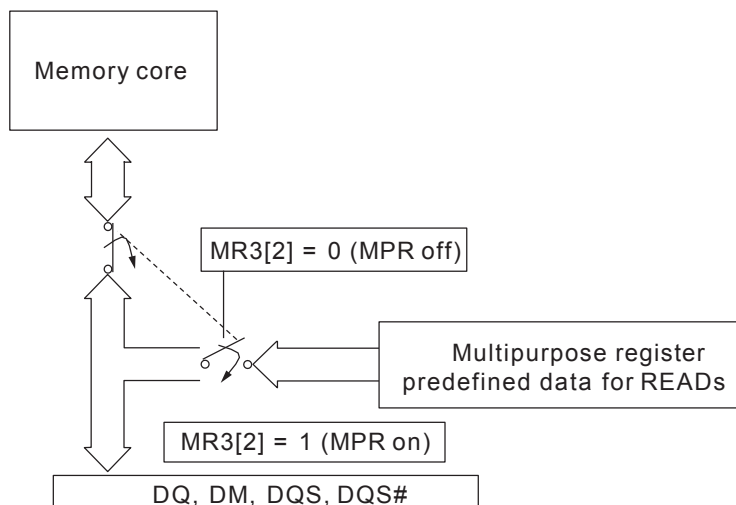
Figure 48 : Multipurpose Register (MPR) Block Diagram
