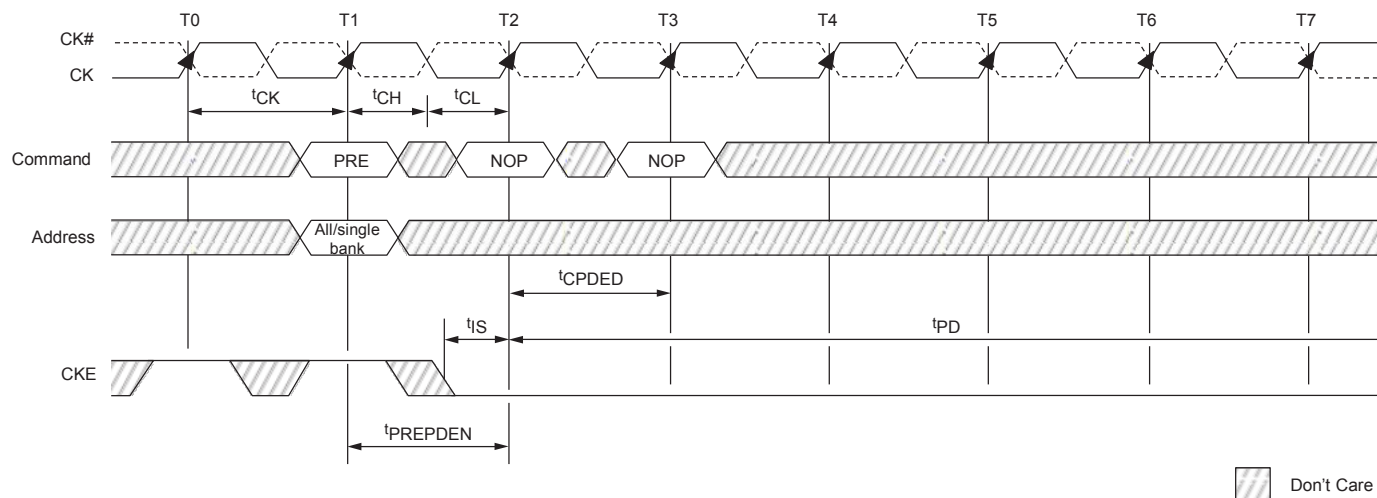
Figure 93 : PRECHARGE to Power-Down Entry
