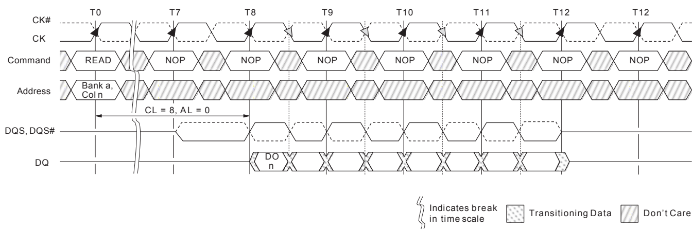
Figure 56 : READ Latency
