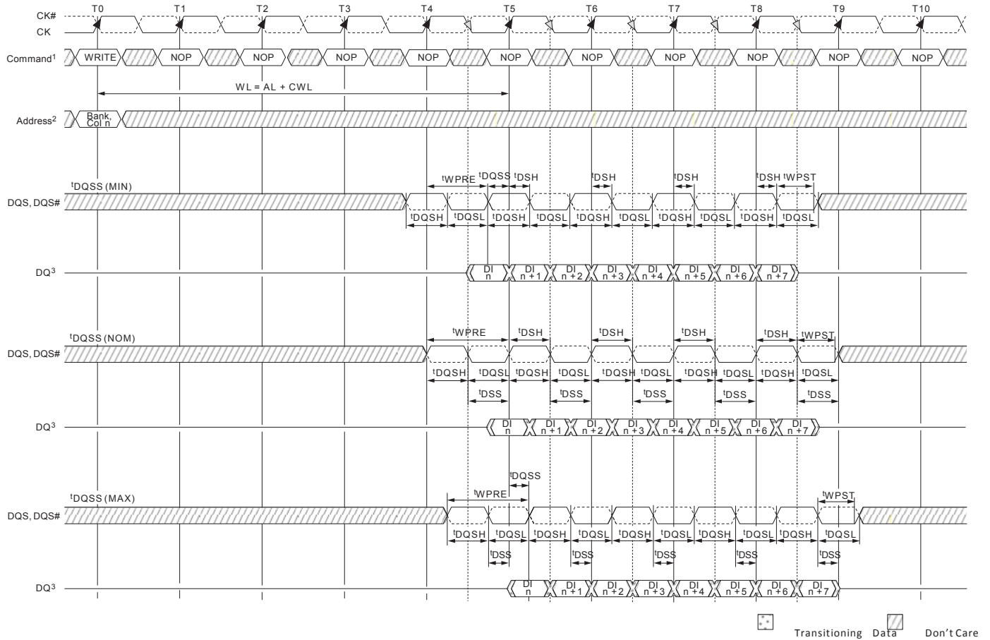
Figure 73 : WRITE Burst
