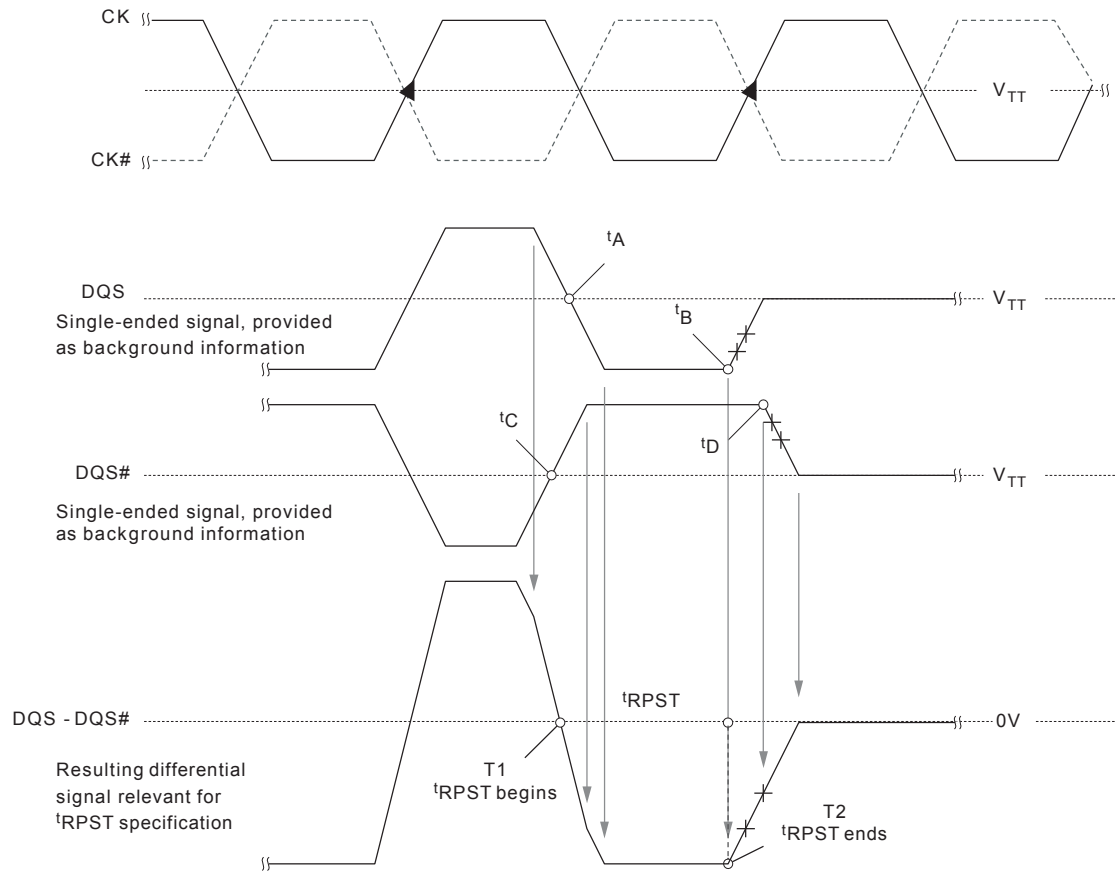
Figure 70 : tRPST Timing
