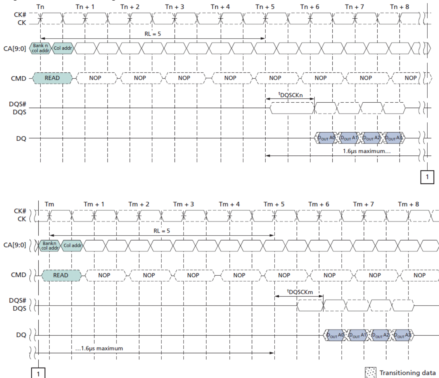
Figure 9 : tDQSKDM Timing
