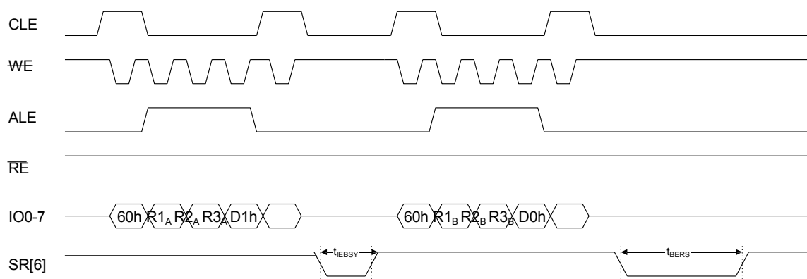
Figure 24: Multiple plane block erase (ONFI 1.0 protocol)
