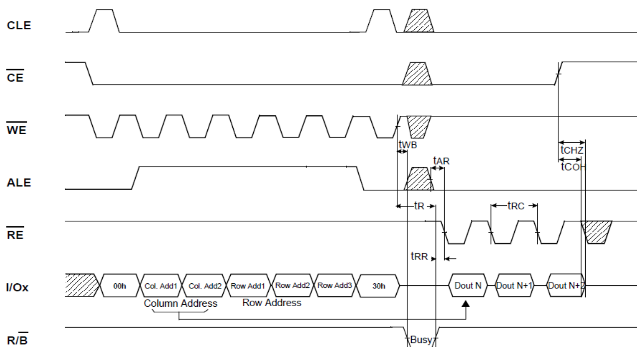
Figure 11 : Read Operation intercepted by \overline{\text{CE}}
