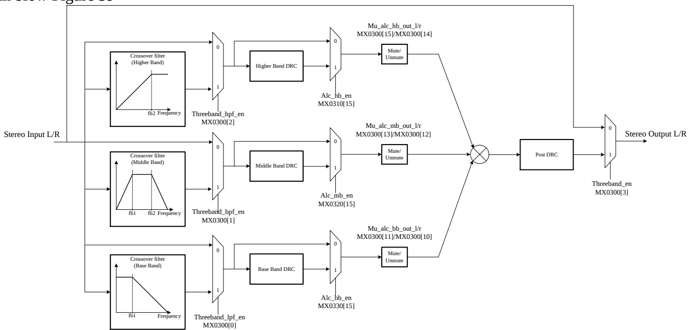
Figure 39. Three-Band DRC Structure
