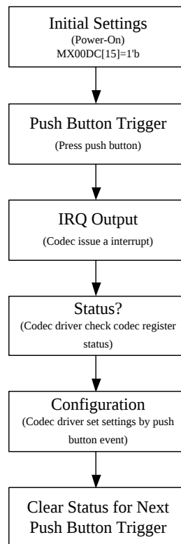
Figure 49. 3 Push Button Detection Flow
