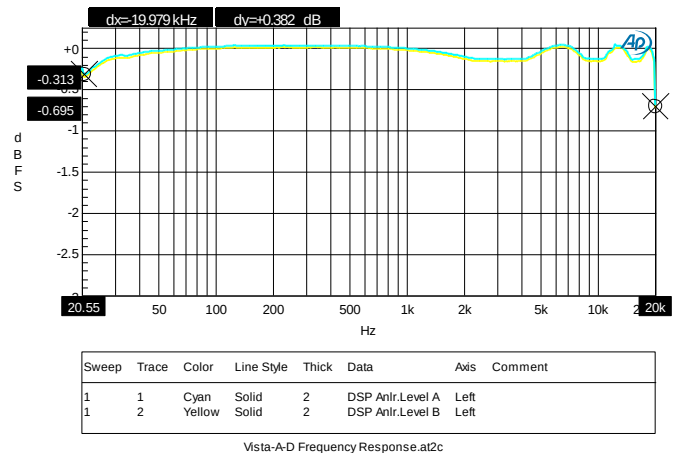
FIGURE 20. 48K/16BIT, LINE IN, FREQUENCY RESPONSE
