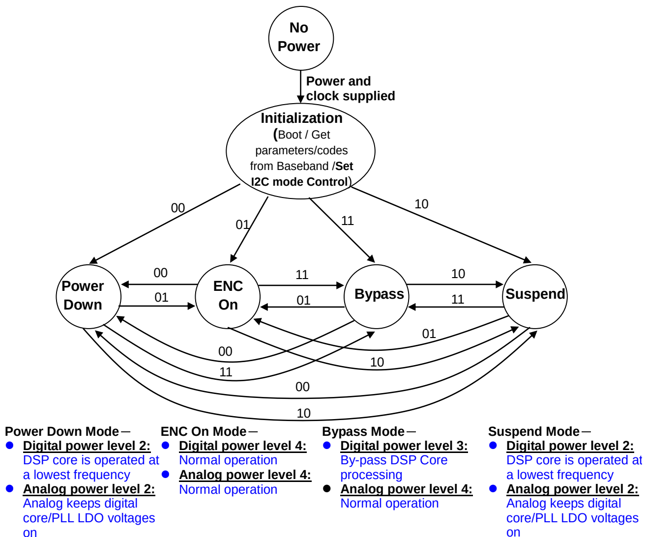
Figure 9.2 Mode State Diagram (by I2C interface)
