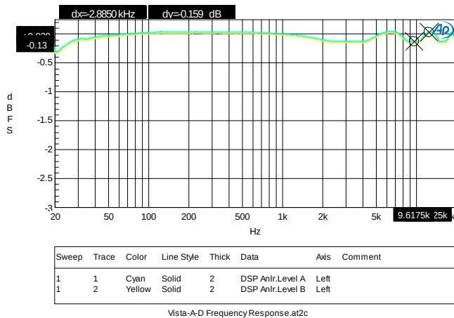
FIGURE 19. 48K/16BIT, LINE IN, PASSBAND RIPPLE
