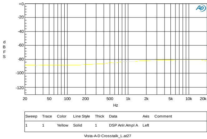
FIGURE 17. 48K/16BIT, MICROPHONE IN, CHANNEL SEPARATION L
