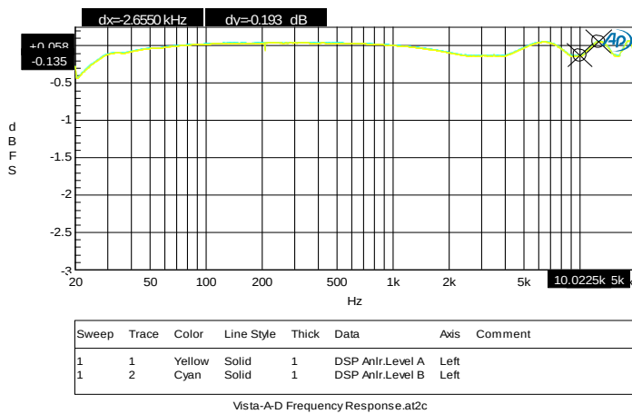
5.2.1.1 PASSBAND RIPPLE 48K FIGURE 15. 48K/16BIT, MICROPHONE IN, PASSBAND RIPPLE
