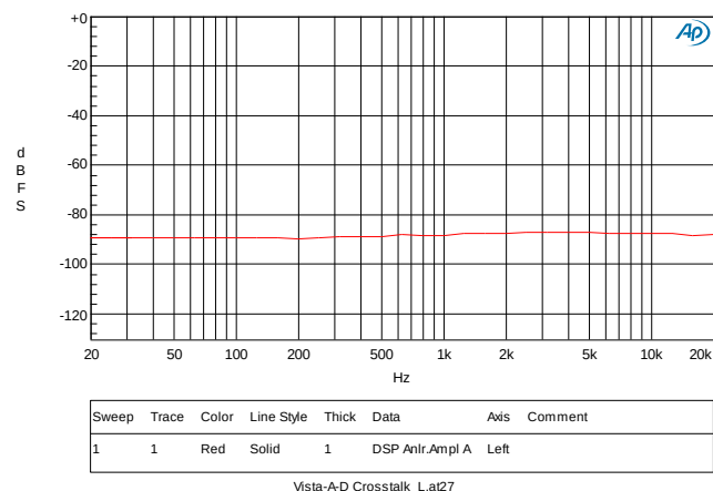
FIGURE 22. 48K/16BIT, LINE IN, CHANNEL SEPARATION L
