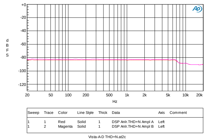
FIGURE 28. 96K/24BIT, LINE IN, THD+N
