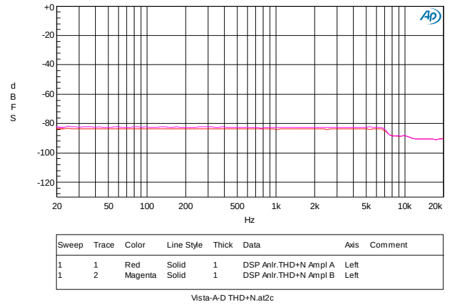
FIGURE 18. 48K/16BIT, LINE IN, THD+N
