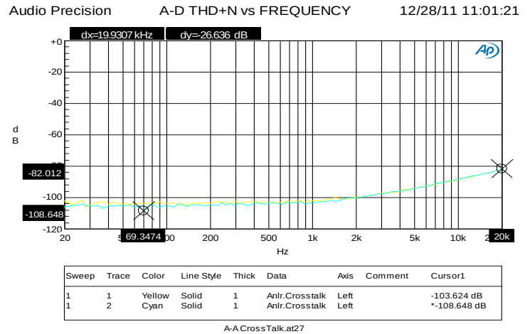
FIGURE 34. LINE IN TO LINE OUT, CROSSTALK L
