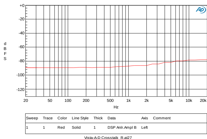
FIGURE 21. 48K/16BIT, LINE IN, CHANNEL SEPARATION R
