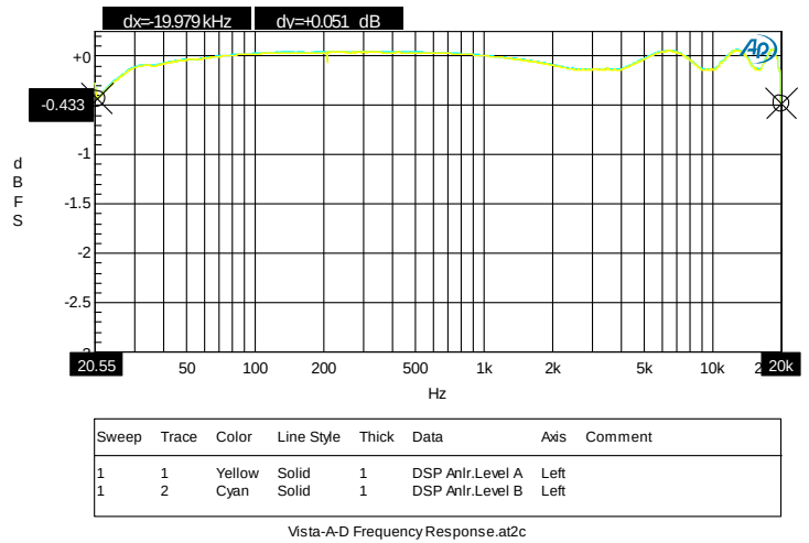
FIGURE 14. 48K/16BIT, MICROPHONE IN, FREQUENCY RESPONSE
