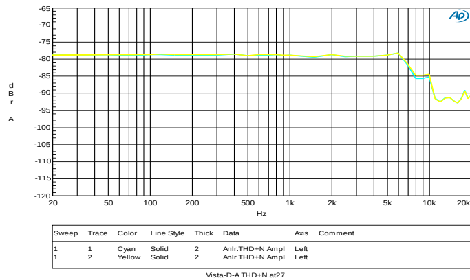
FIGURE 1. 48k/16BIT, 10K LOADING DAC, THD+N
