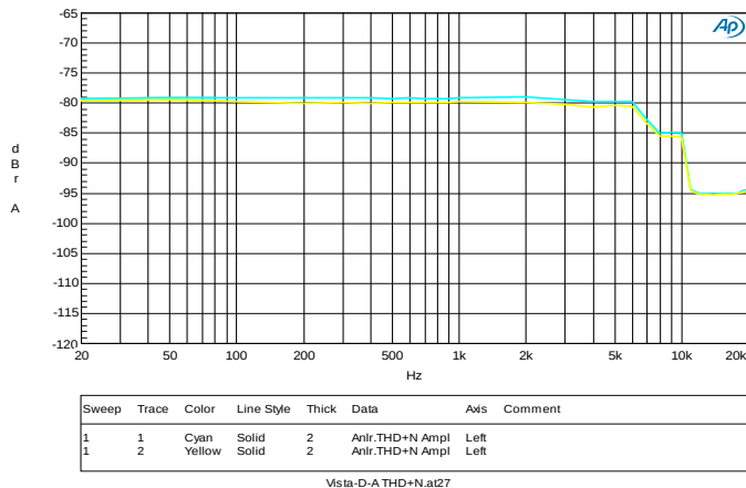
FIGURE 7. 96k/24BIT, 10K LOADING DAC, THD+N
