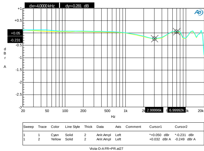
FIGURE 3. 48k/16BIT, 10K LOADING DAC, PASSBAND RIPPLE
