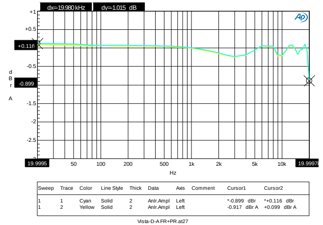
FIGURE 2. 48k/16BIT, 10K LOADING DAC, FREQUENCY RESPONSE
