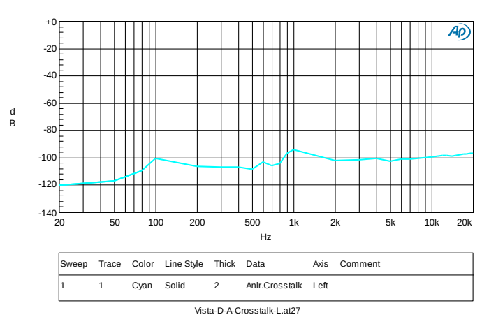
FIGURE 10. 96k/24BIT, 10K LOADING DAC, CROSSTALK L
