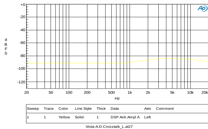
FIGURE 27. 96K/24BIT, MICROPHONE IN, CHANNEL SEPARATION L
