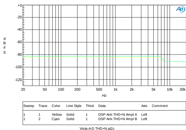
FIGURE 23. 96K/24BIT, MICROPHONE IN, THD+N
