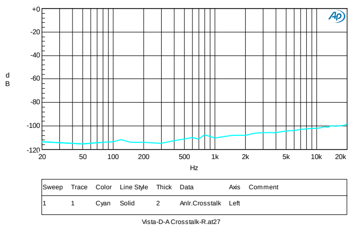
FIGURE 4. 48k/16BIT, 10K LOADING DAC, CROSSTALK L
