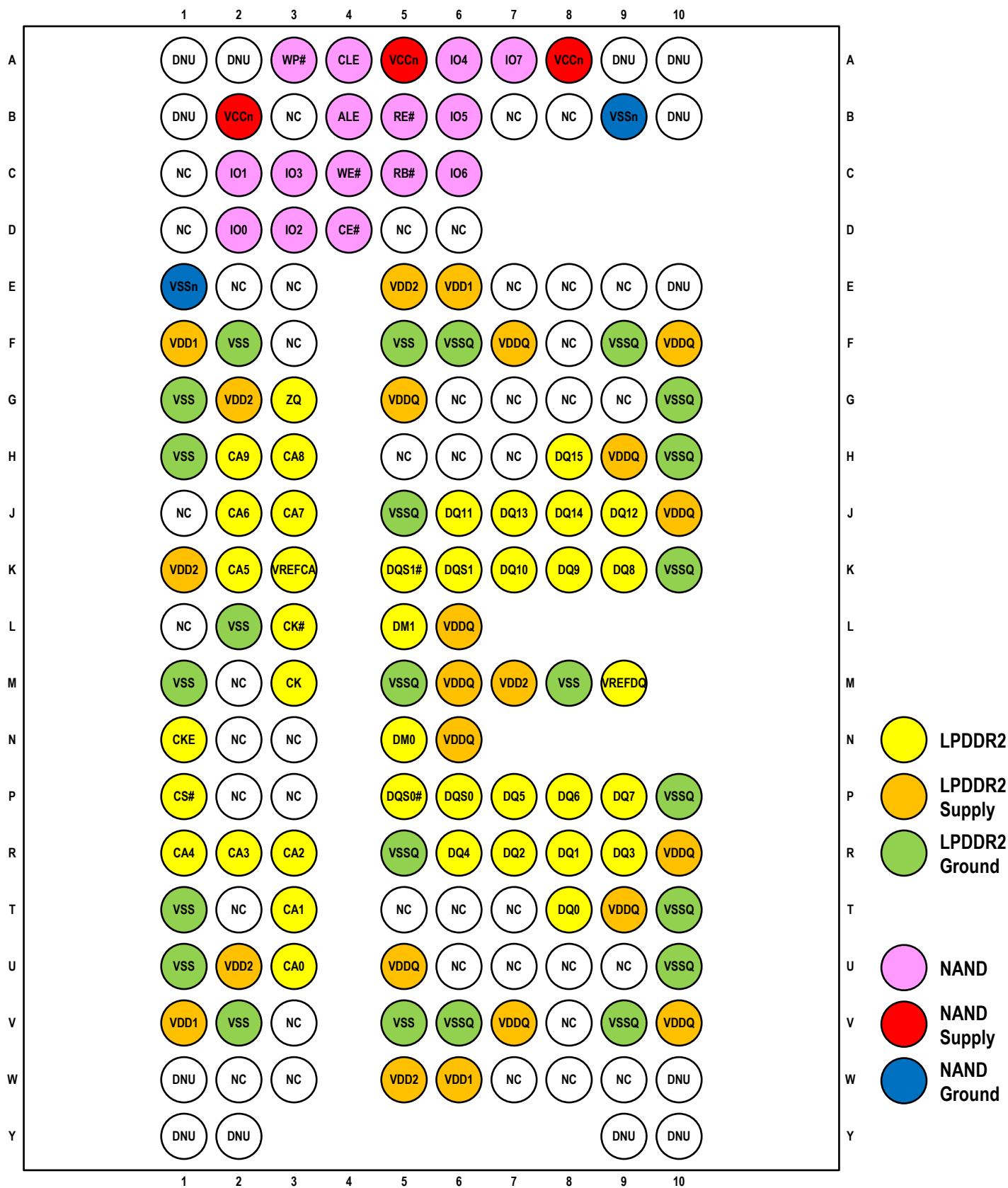
Pin Configuration – 162Ball MCP(X8/X16)
