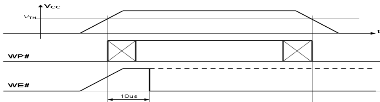
Figure 31 : Power on and Data Protection timings
