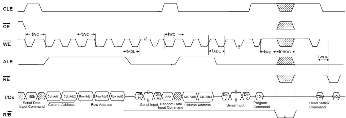
Figure 16 : Random Data In
