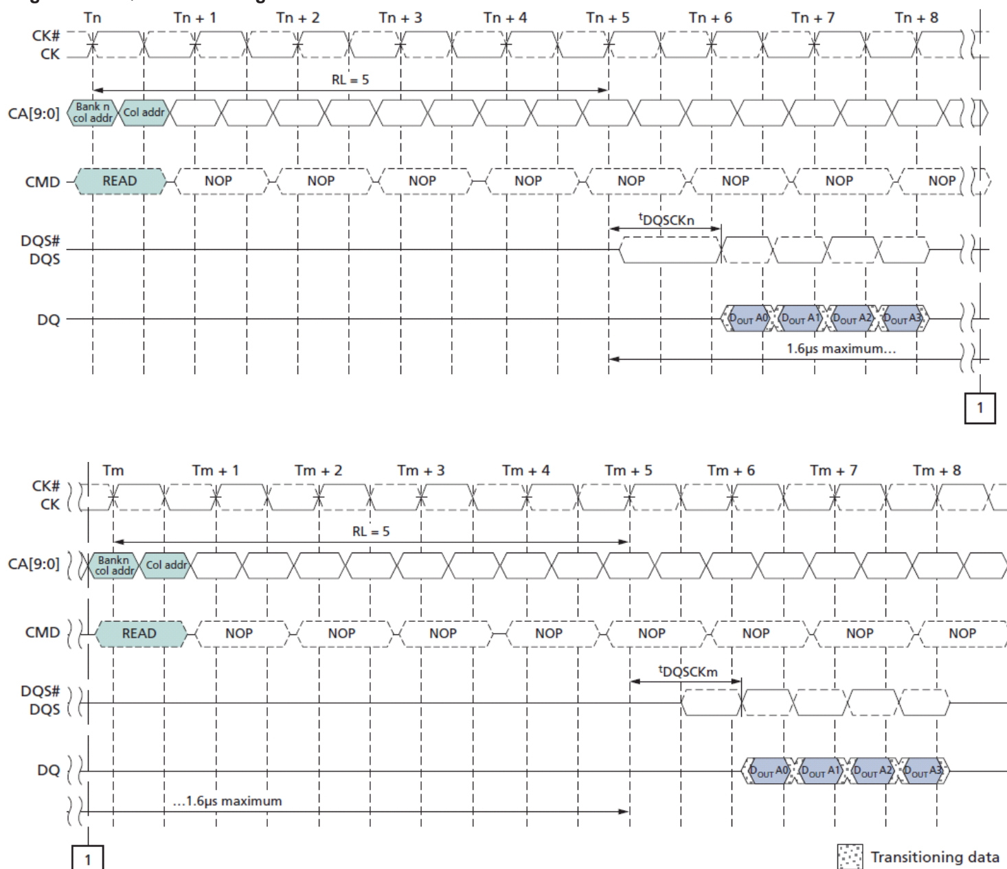
Figure 9 : tDQSKDM Timing
