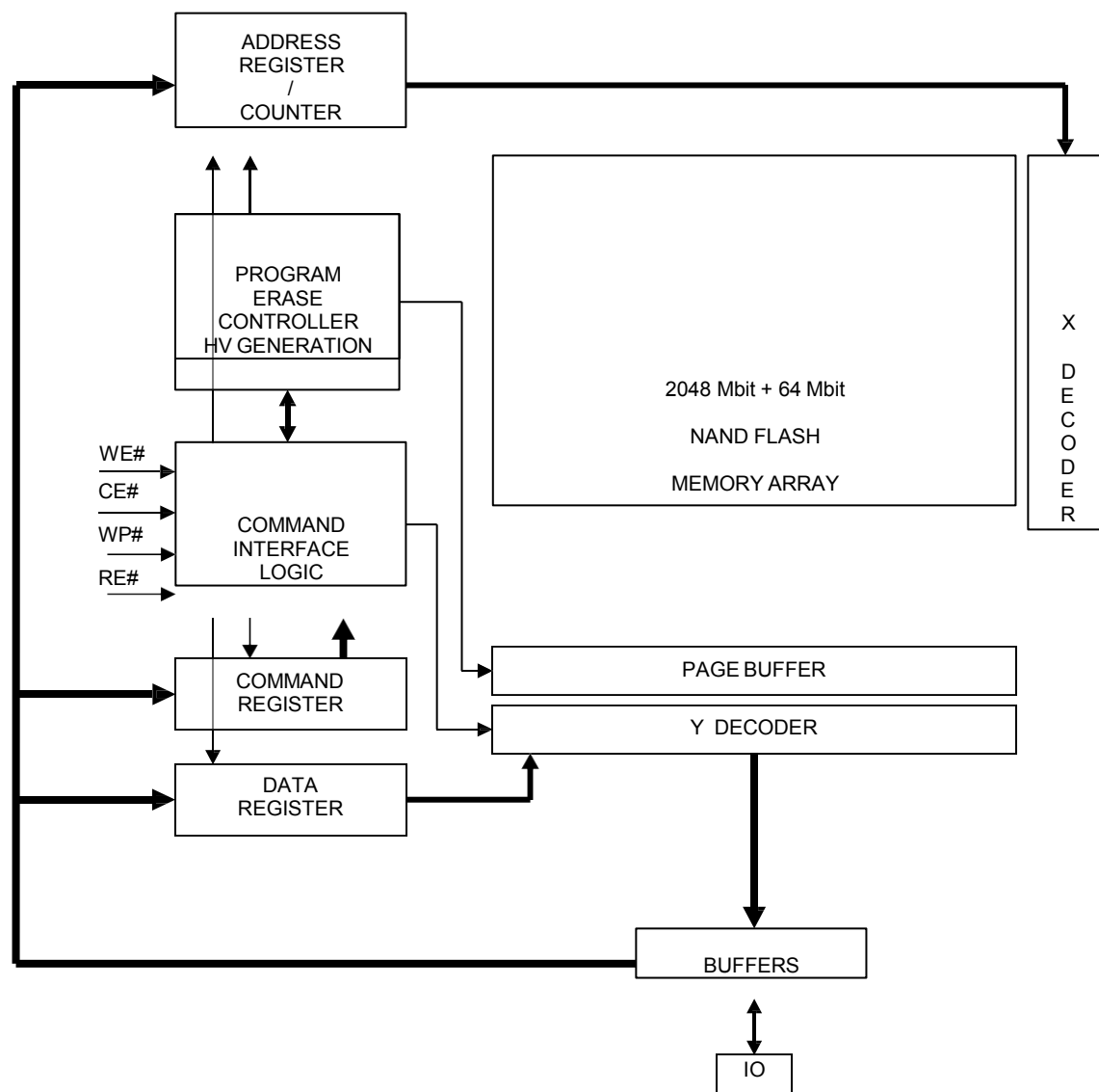
Figure 2 : block description
