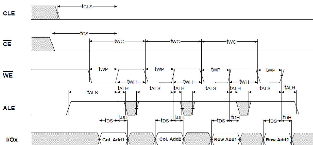
Figure 4 : Address Latch Cycle
