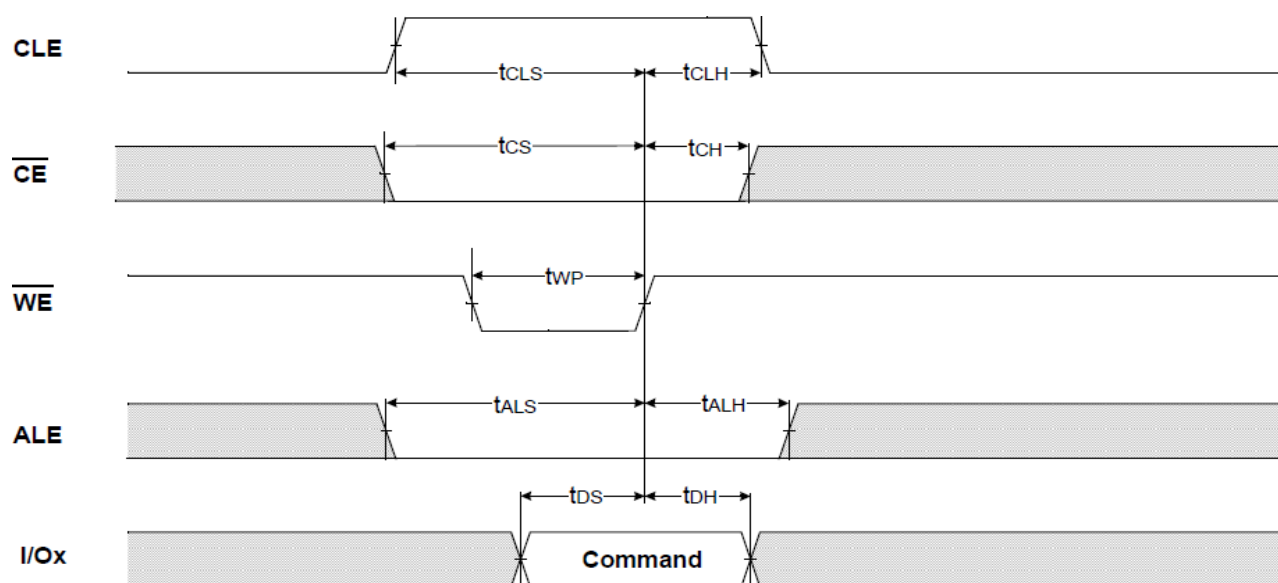
Figure 3 : Command Latch Cycle
