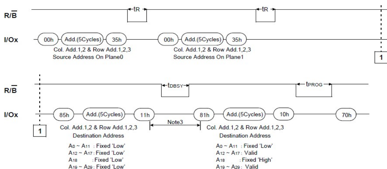
Figure 19 : multi-plane copyback program
