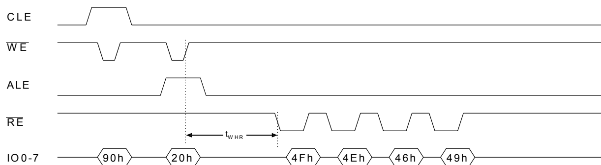
Figure 26 : ONFI signature timing diagram
