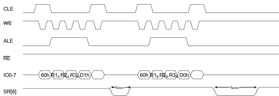
Figure 24: Multiple plane block erase (ONFI 1.0 protocol)
