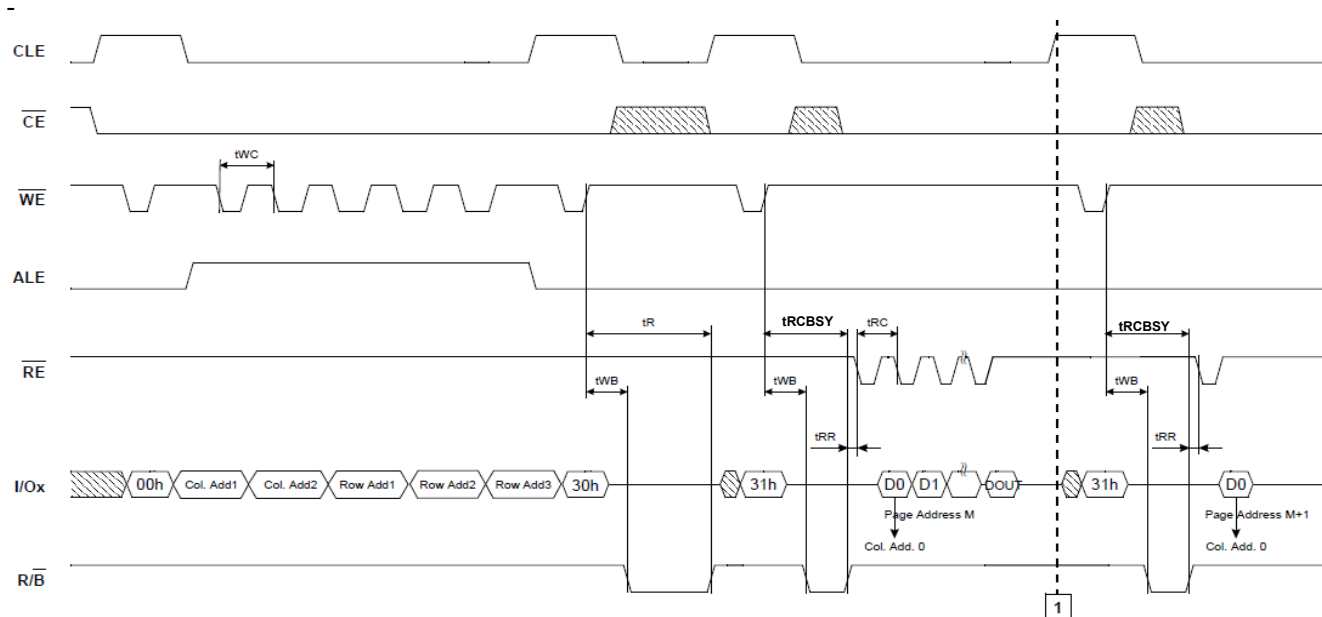
Figure 13 : read cache timings, start of cache operation
