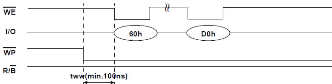
Figure 30 : t_{WW} in Erase Operation
