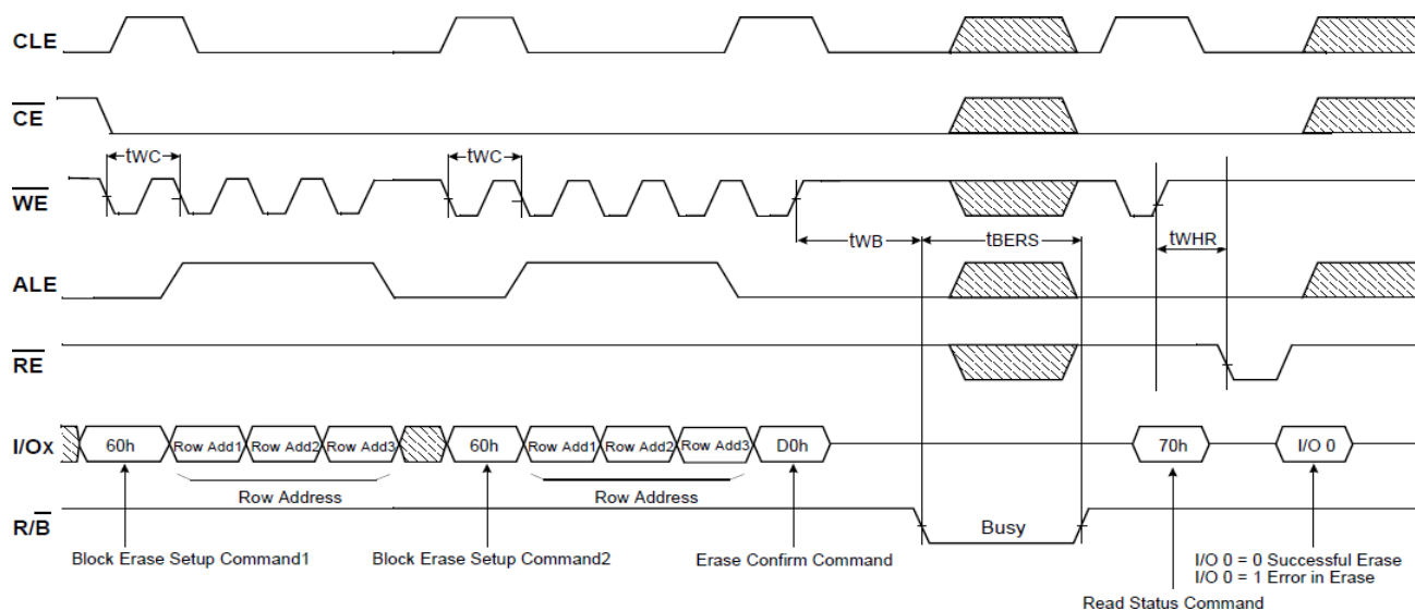
Figure 23 : multi-plane block erase
