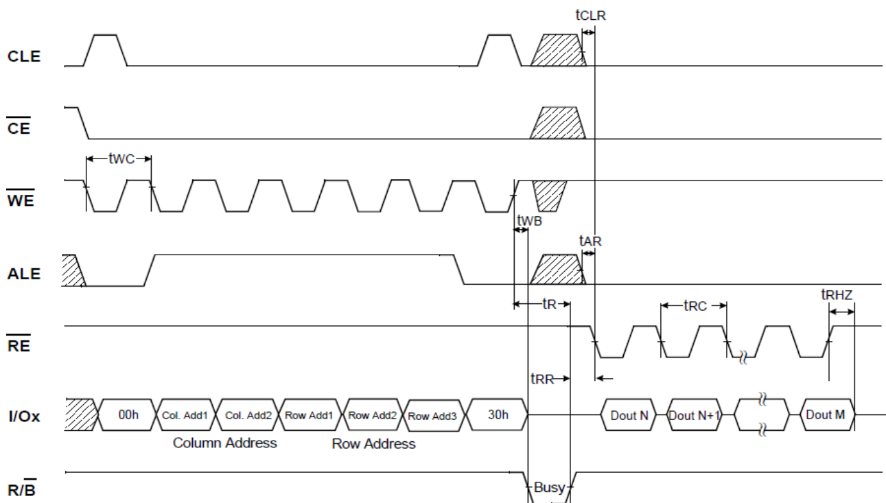
Figure 10 : Read Operation (Read One Page)
