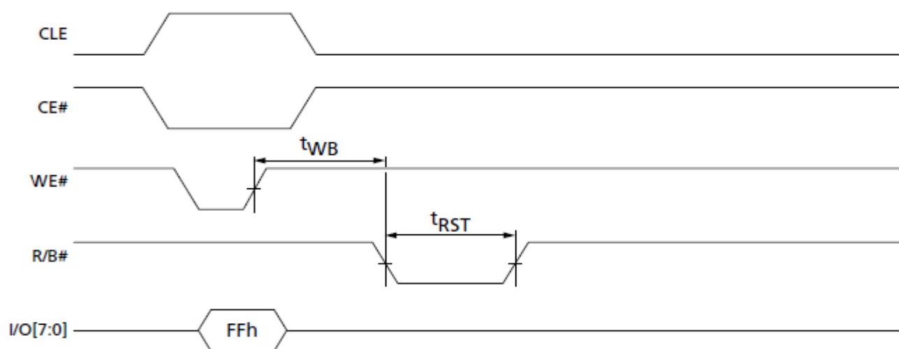
Figure 27 : Reset operation timing
