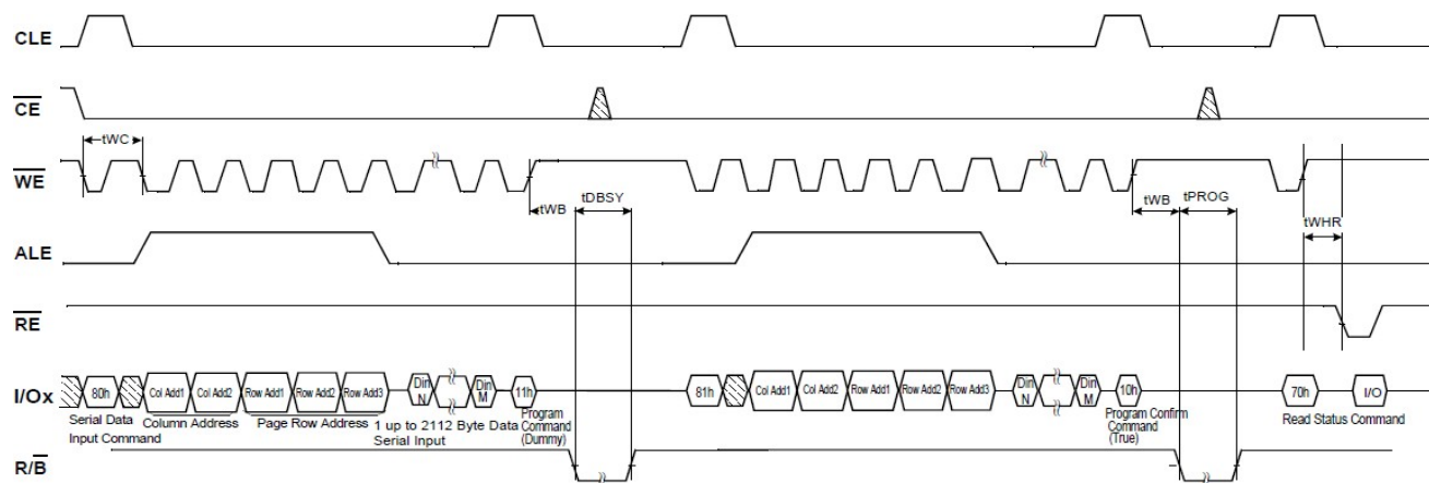
Figure 17 : multi-plane program
