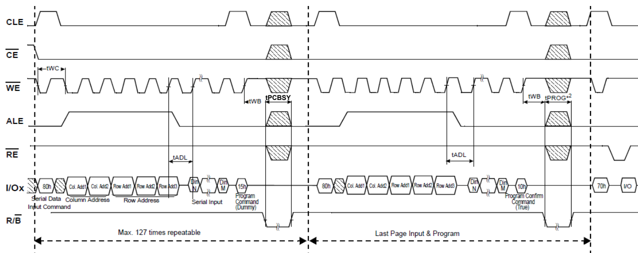
Figure 20 : cache program
