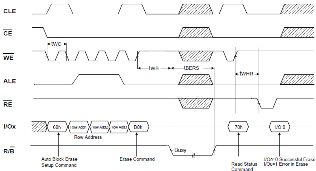
Figure 22 : Block Erase Operation (Erase One Block)
