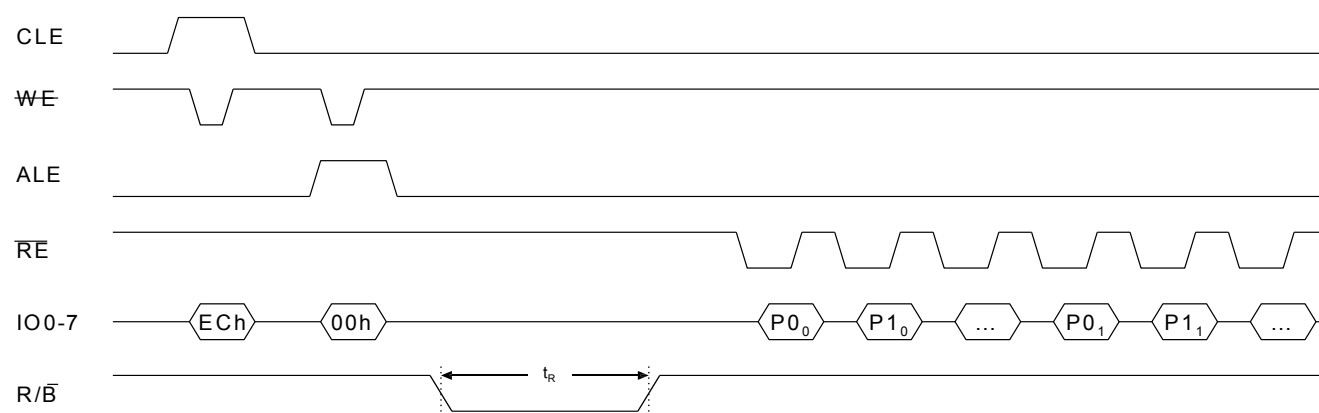
Figure 28 : Read Parameter Page timings
