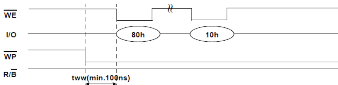
Figure 29 : t_{WW} in Program Operation
