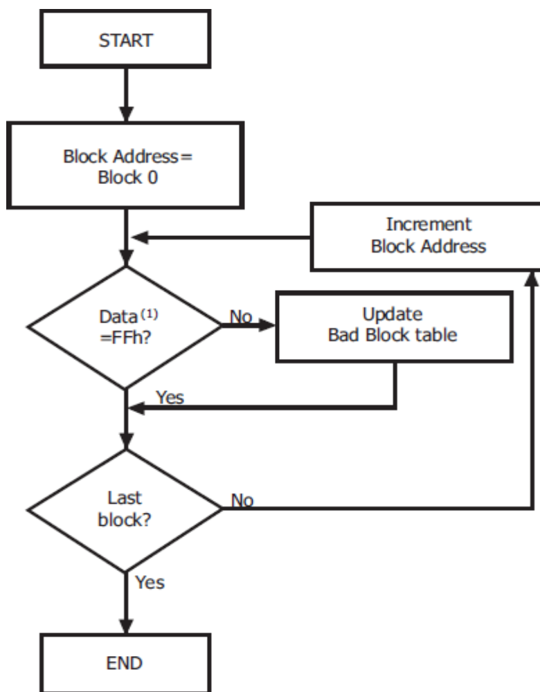
Figure 33 : Bad Block Management Flowchart
