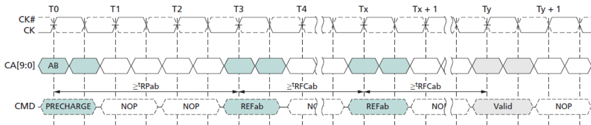
Figure 33 All-Bank REFRESH Operation
