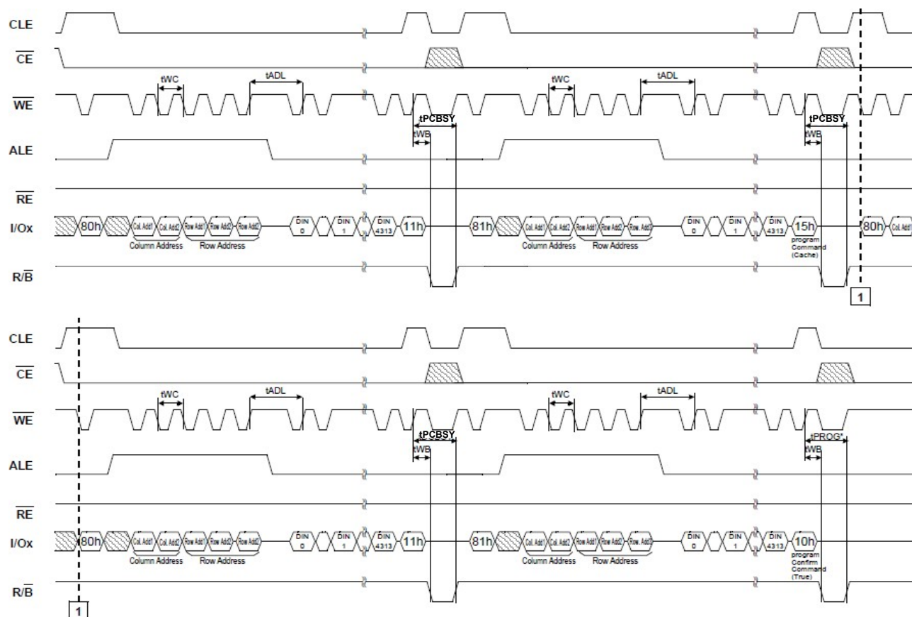
Figure 21 : multi-plane cache program
