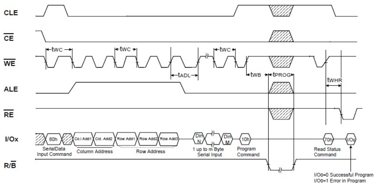
Figure 15 : Page Program Operation
