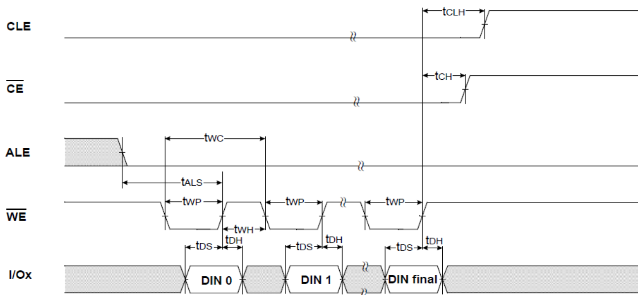
Figure 5 : Input Data Latch Cycle
