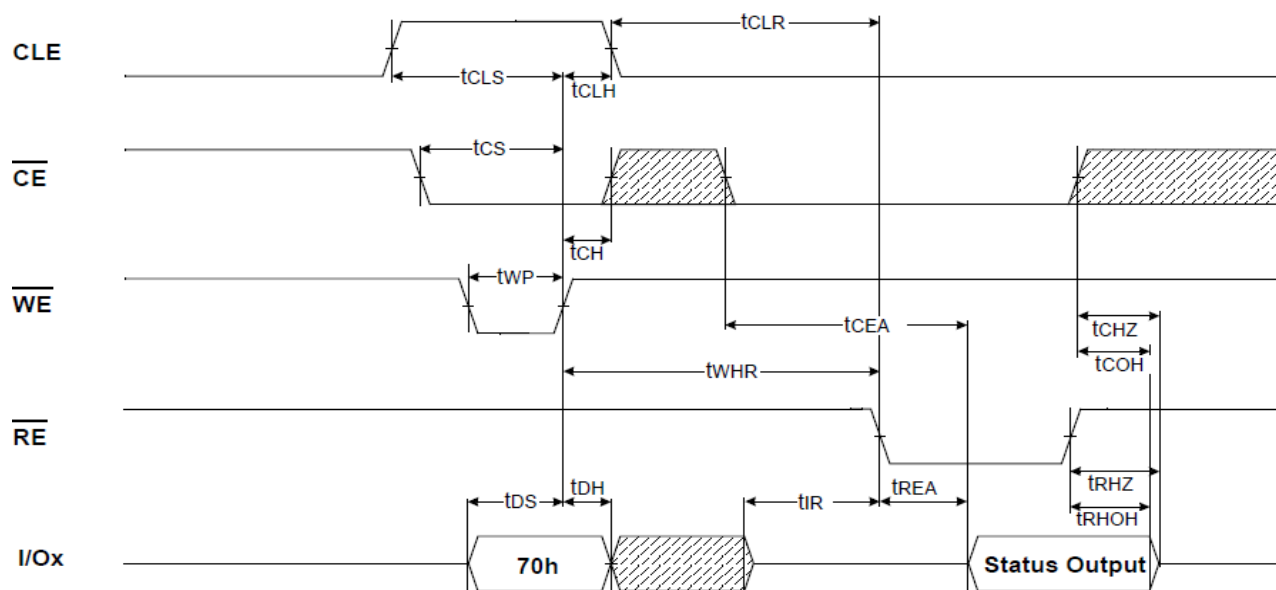
Figure 8 : Status Read Cycle
