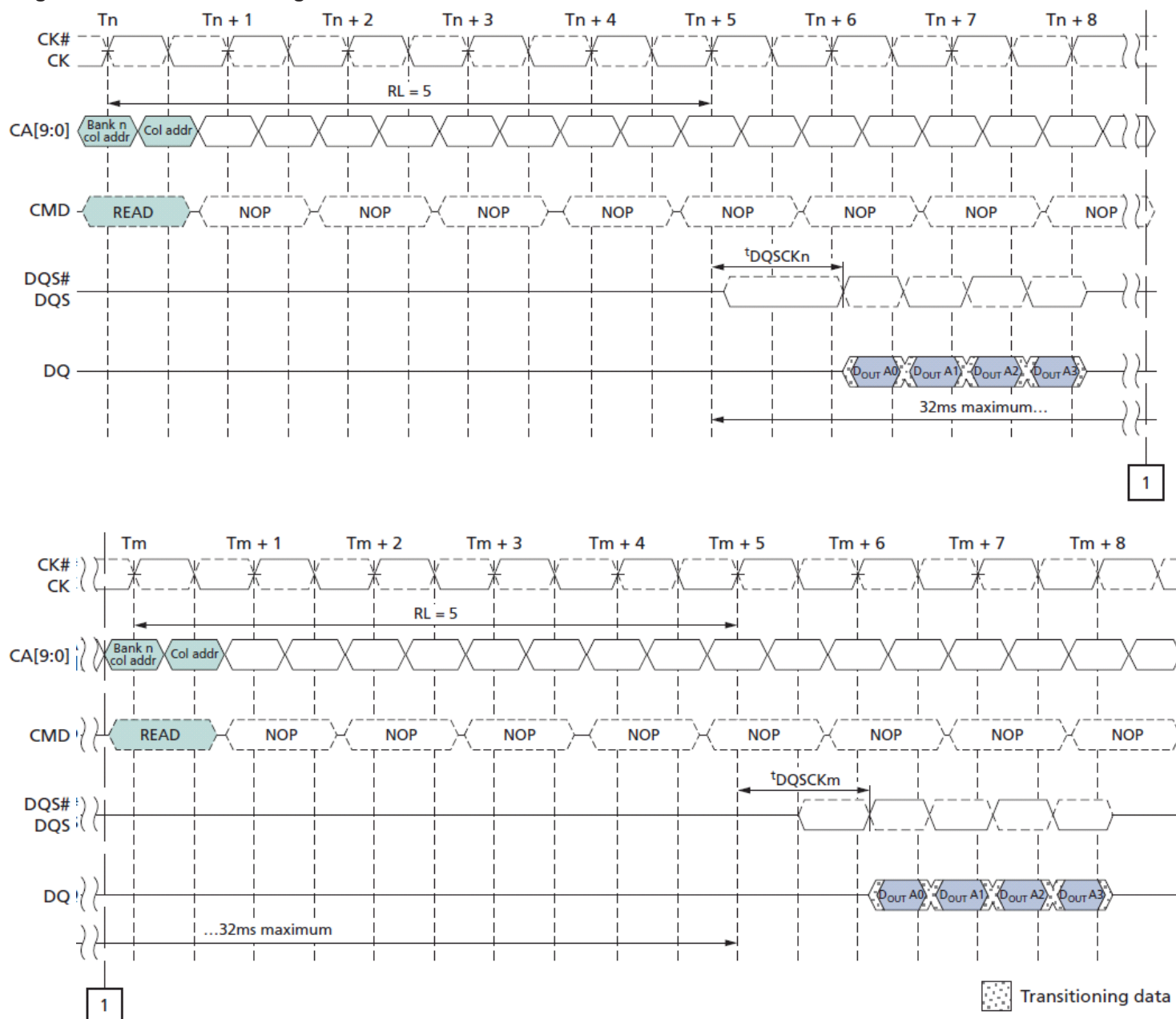
Figure 8 : tDQSKDL Timing
