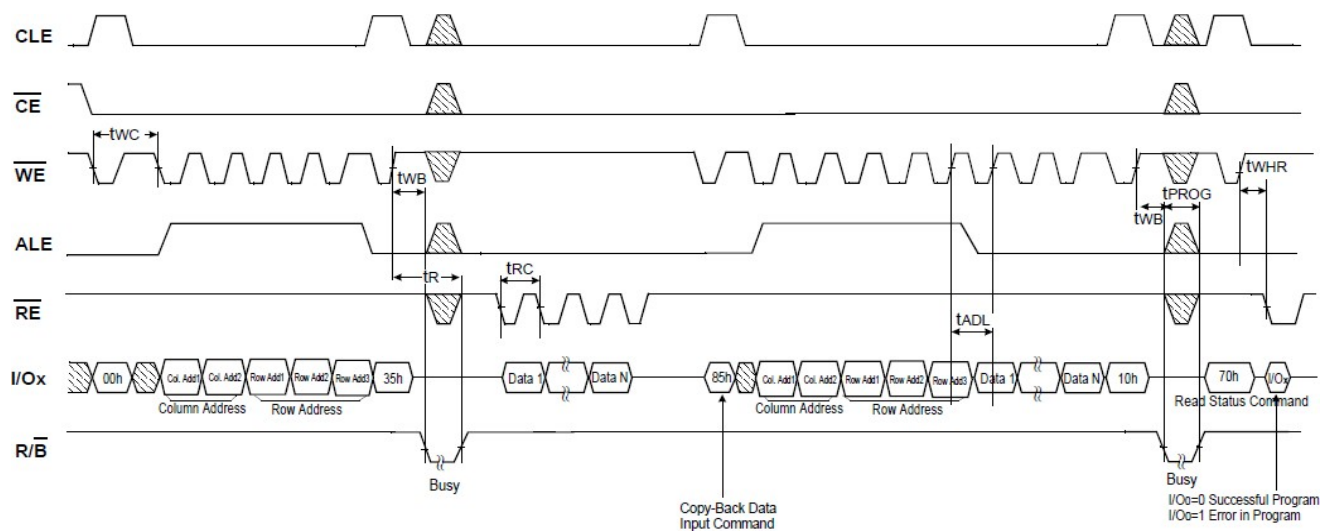
Figure 18 : Copy Back read with optional data readout /Copy back program with optional data input
