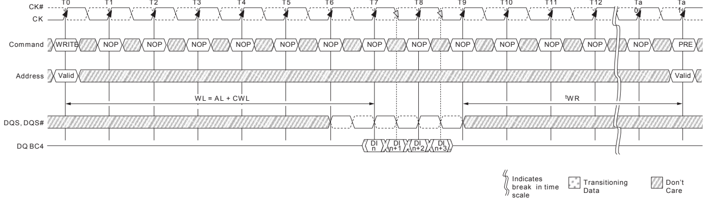
Figure 80 : WRITE (BC4 Mode Register Setting) to PRECHARGE
