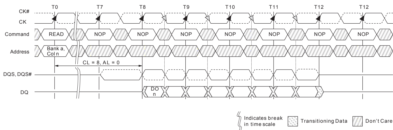
Figure 55 : READ Latency
