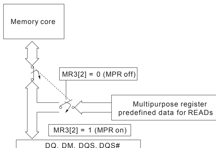
Figure 47 : Multipurpose Register (MPR) Block Diagram
