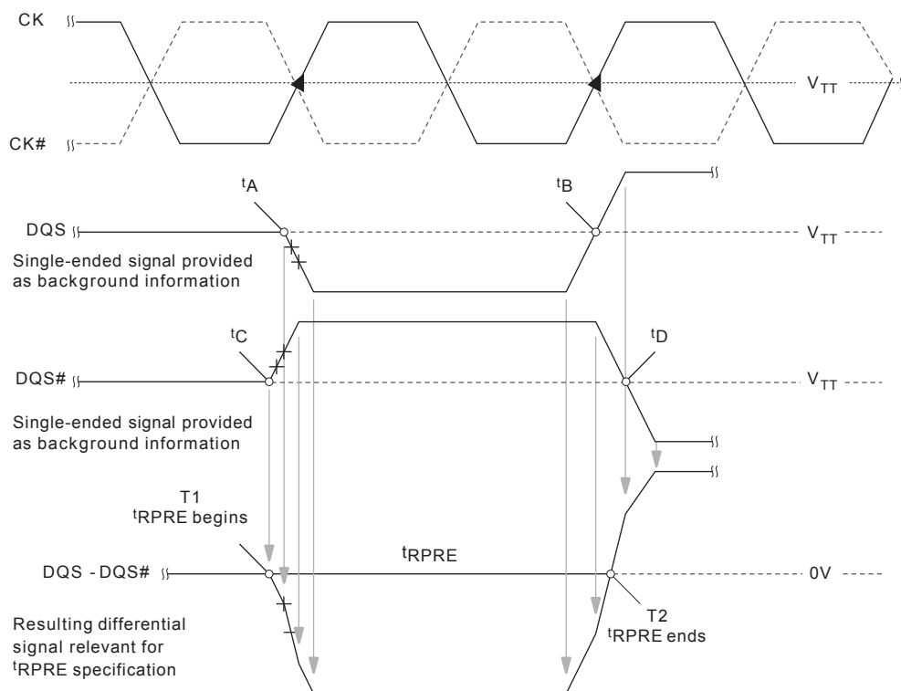
Figure 68 : tRPRE Timing
