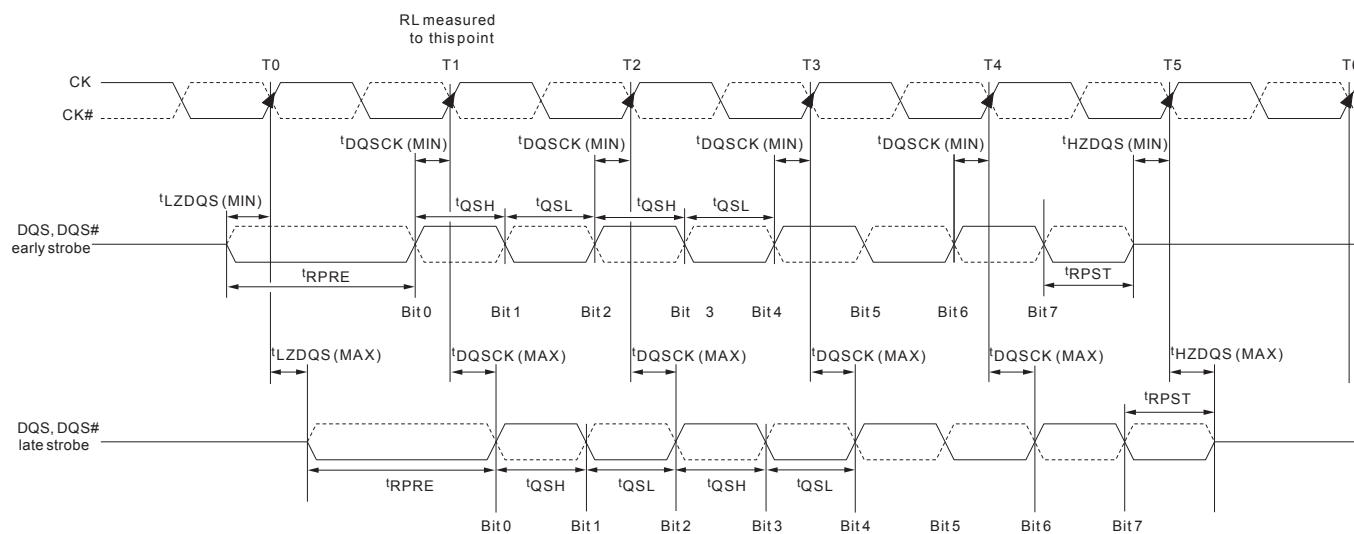
Figure 66 : Data Strobe Timing – READs
