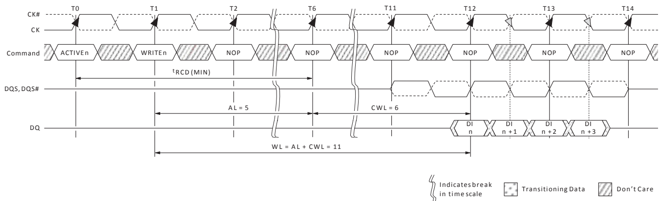
Figure 45 : CAS Write Latency
