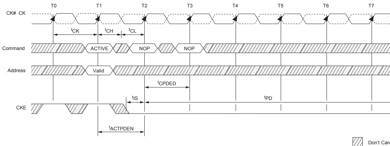
Figure 91 : ACTIVATE to Power-Down Entry
