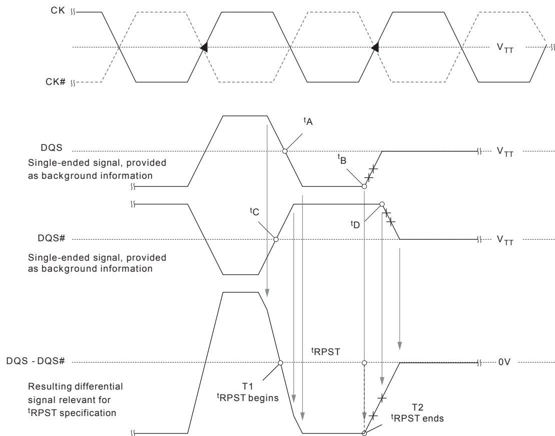
Figure 69 : tRPST Timing
