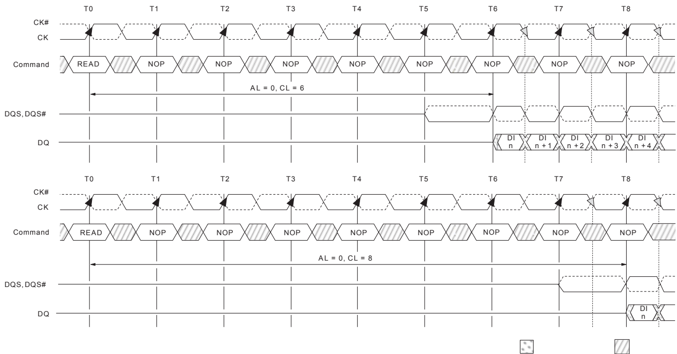
Figure 41 : READ Latency
