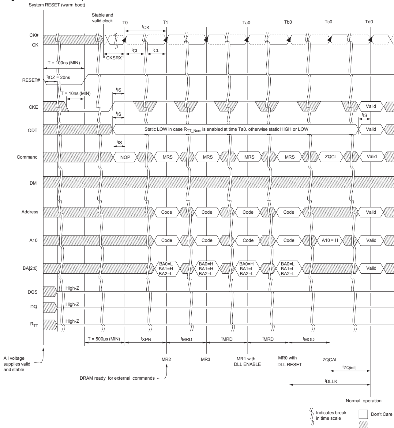
Figure 95 : RESET Sequence
