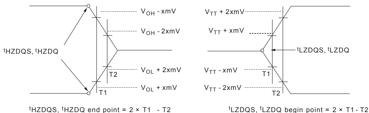
Figure 67 : Method for Calculating tLZ and tHZ
