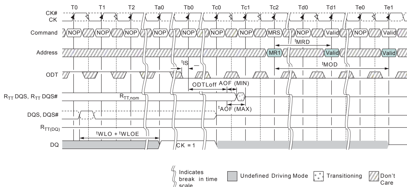
Figure 36 : Write Leveling Exit Procedure
