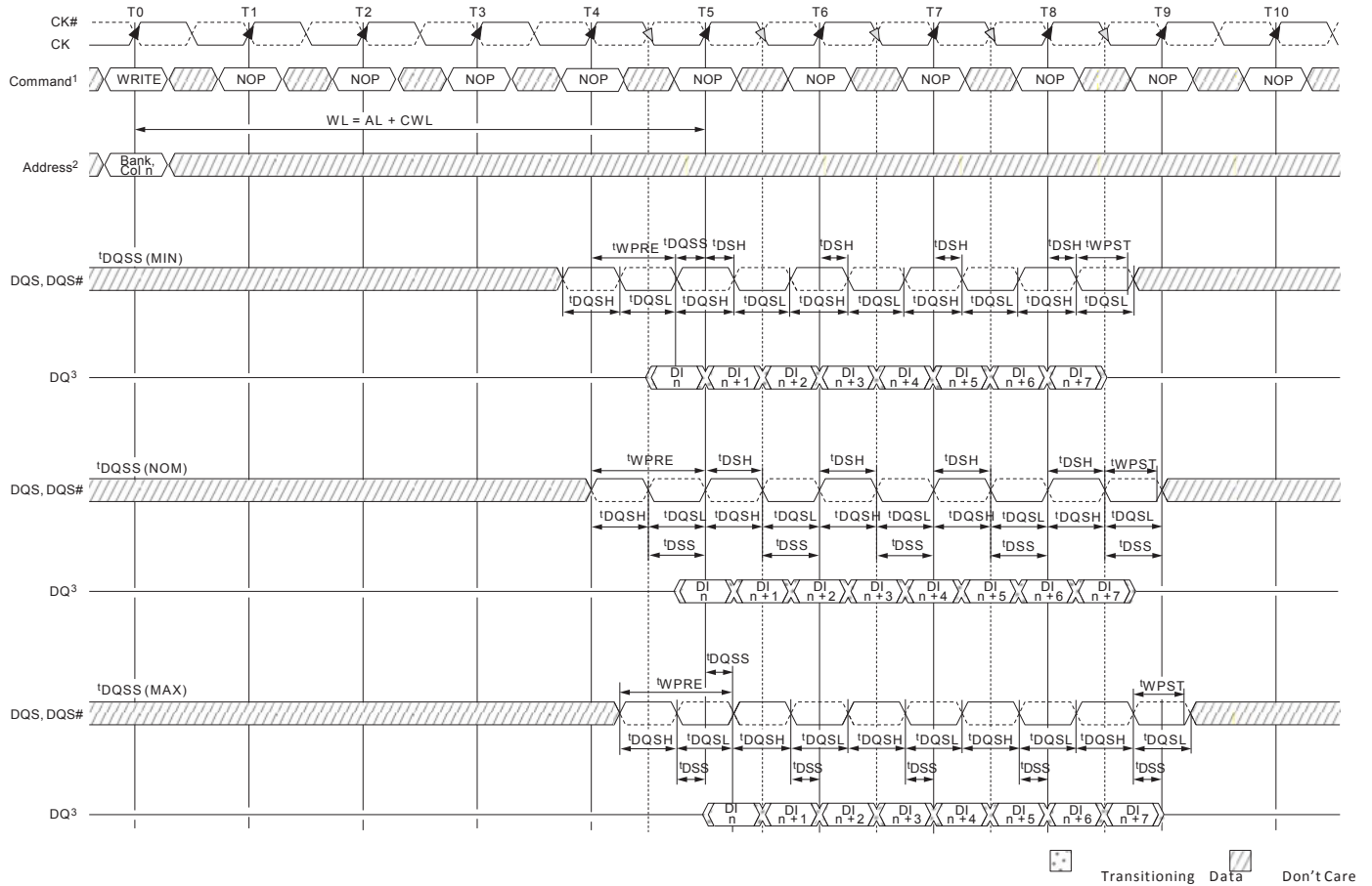
Figure 72 : WRITE Burst
