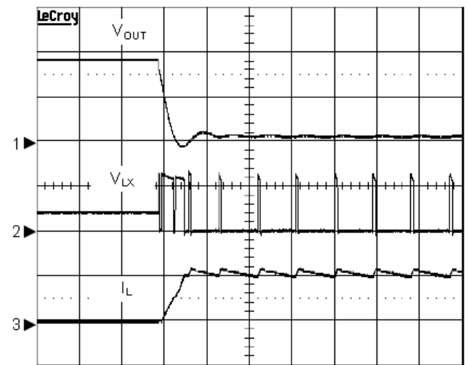
Short Circuit
