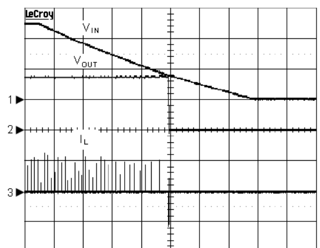
Power Off
