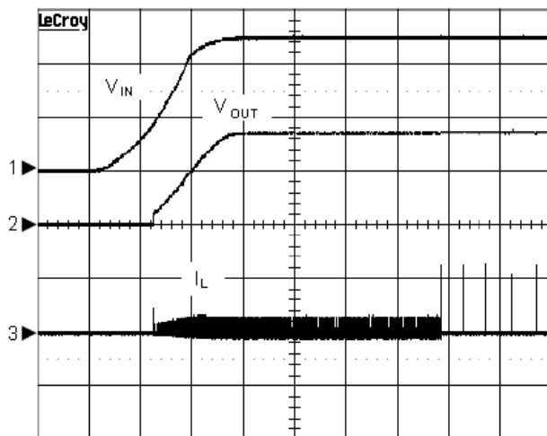
Power On
