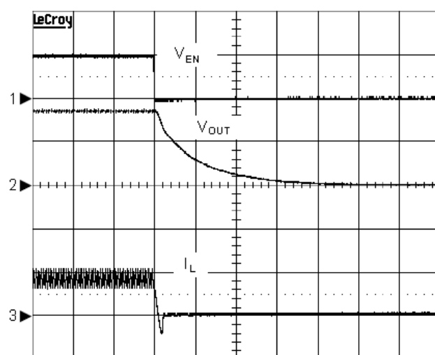
Shutdown
