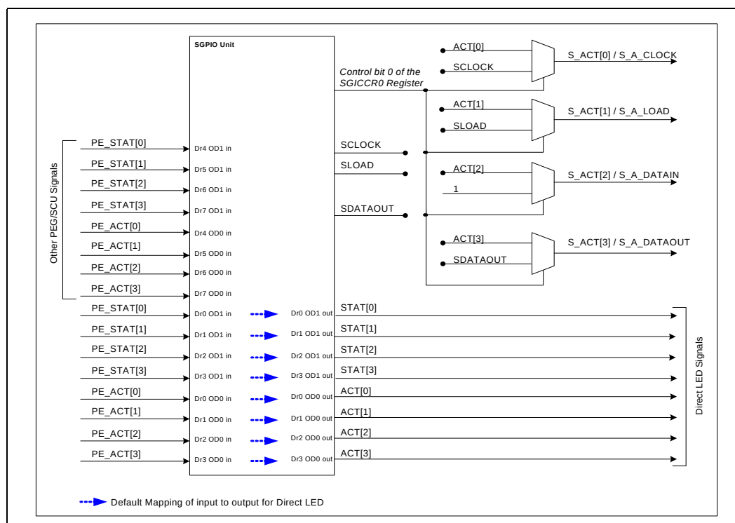
Figure 5-28. SCU SGPIO Unit Pin Mapping
