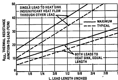
FIGURE 11 - STEADY-STATE THERMAL RESISTANCE
