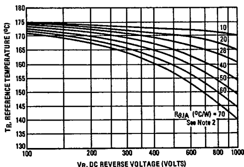
FIGURE 1 - MAXIMUM REFERENCE TEMPERATURE
