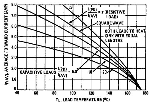
FIGURE 5 - 1/8" LEAD LENGTH
