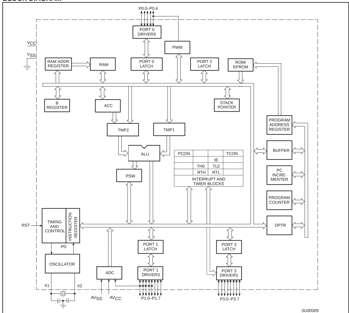
BLOCK DIAGRAM
