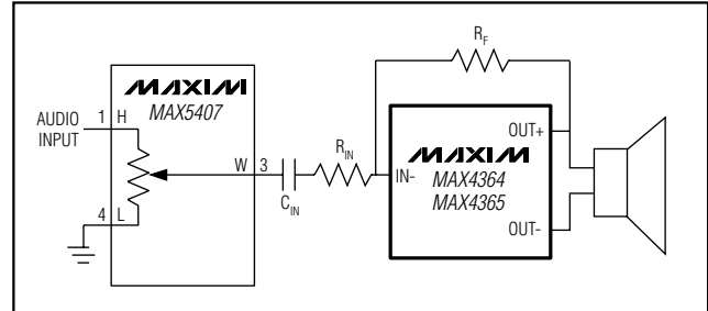
Figure 3. MAX4364/MAX4365 and MAX5160 Volume Control Circuit
