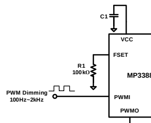
Figure 4—Direct PWM Dimming with Positive Logic
