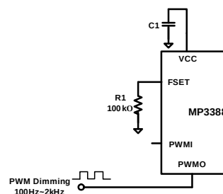
Figure 5—Direct PWM Dimming with Negative Logic
