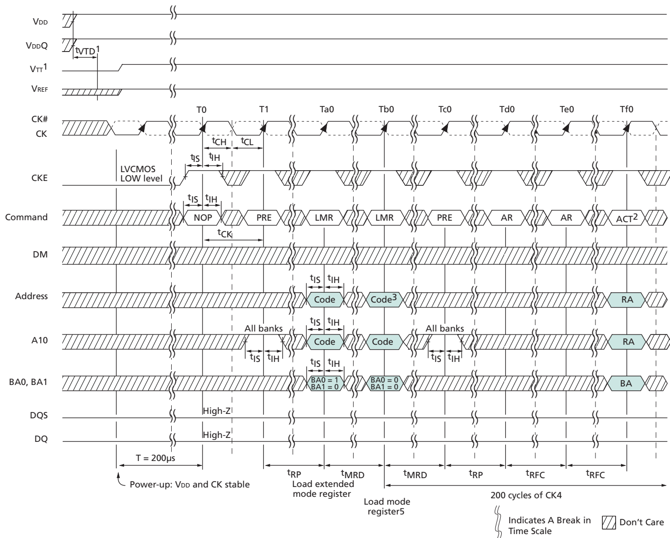
Figure 23: INITIALIZATION Timing Diagram
