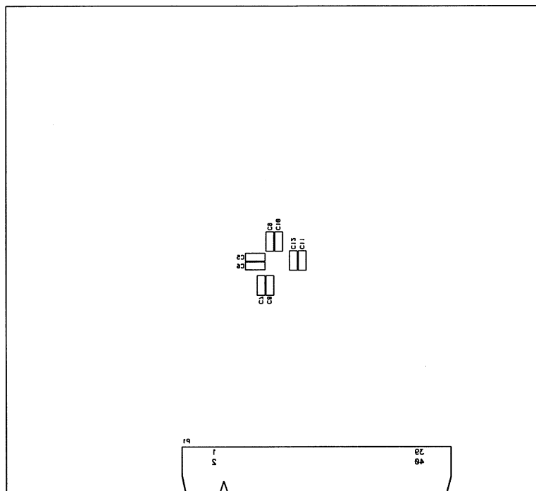
Figure 44. Silkscreen Layer—Bottom
