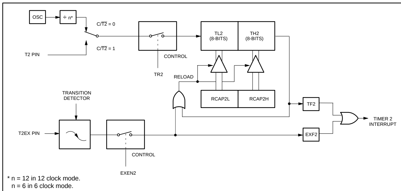
Figure 5 : Timer 2 in Auto-Reload Mode (DCEN = 0)
