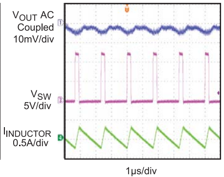
Switching Waveform
