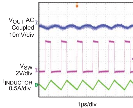
Switching Waveform
