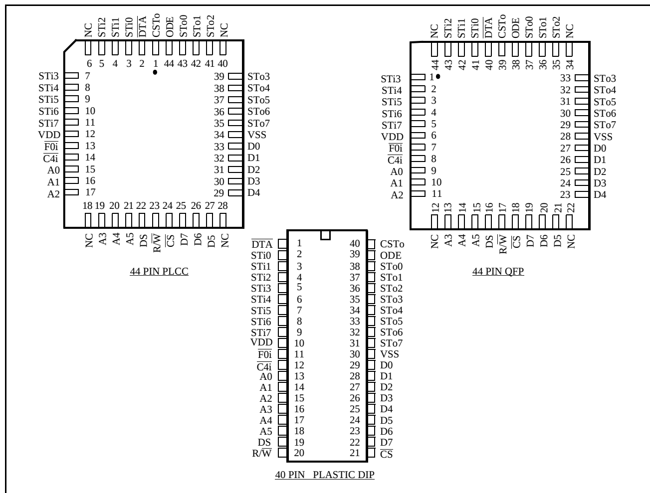
Figure 2 - Pin Connections
