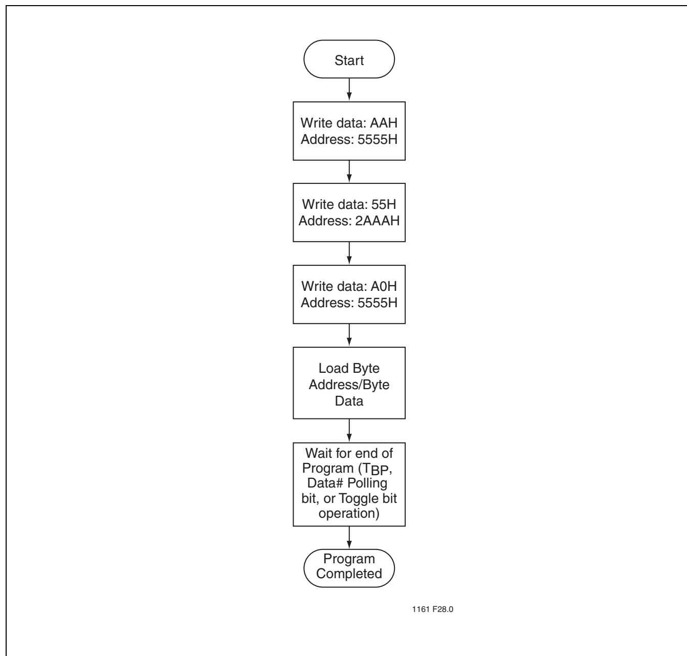
FIGURE 25: Byte-Program Algorithm
