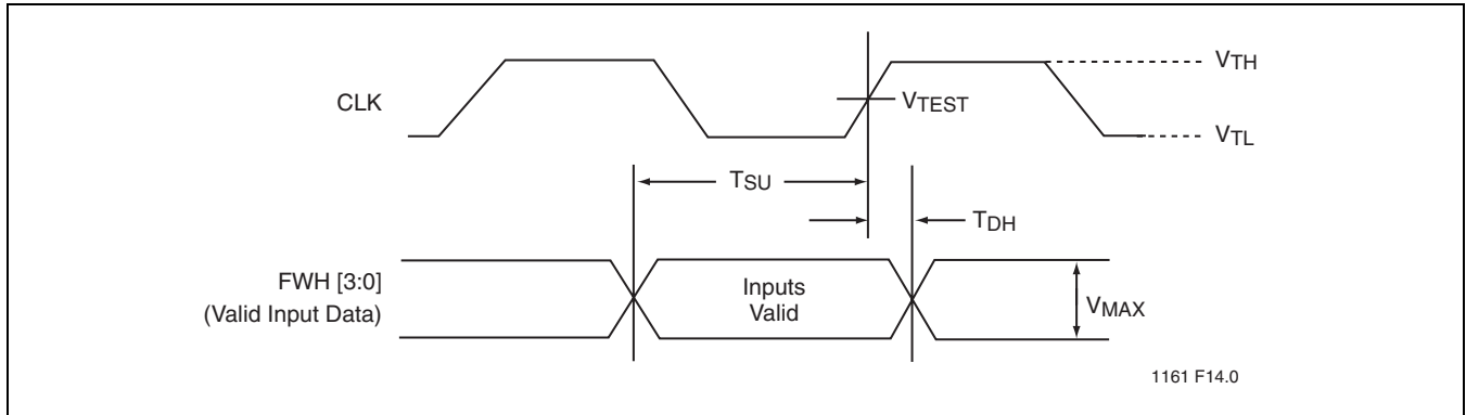
FIGURE 11: Input Timing Parameters
