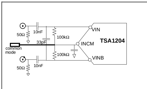
Figure 4 : AC-coupled differential input
