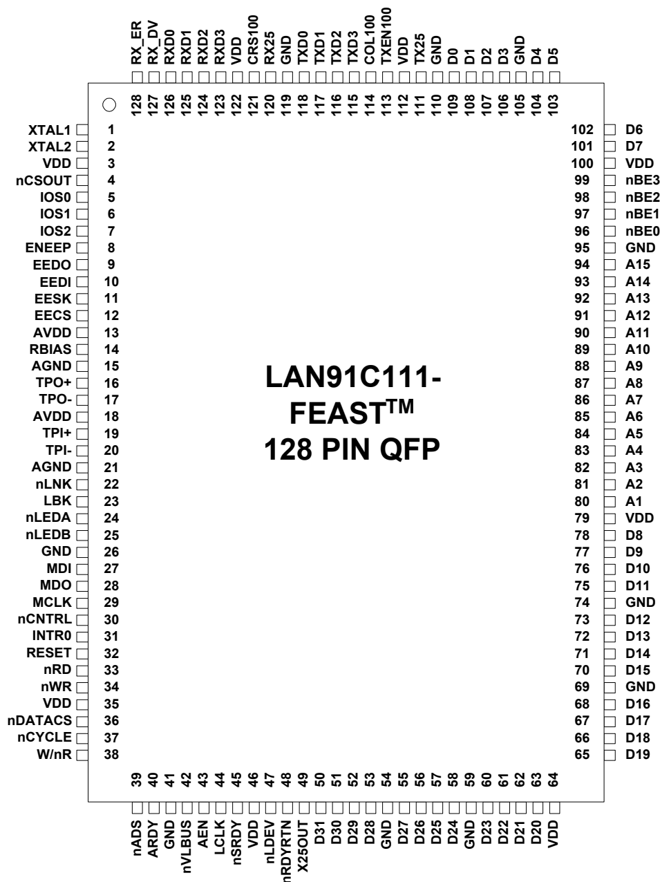
Figure 2.2 Pin Configuration - LAN91C111-FEAST 128 PIN QFP
